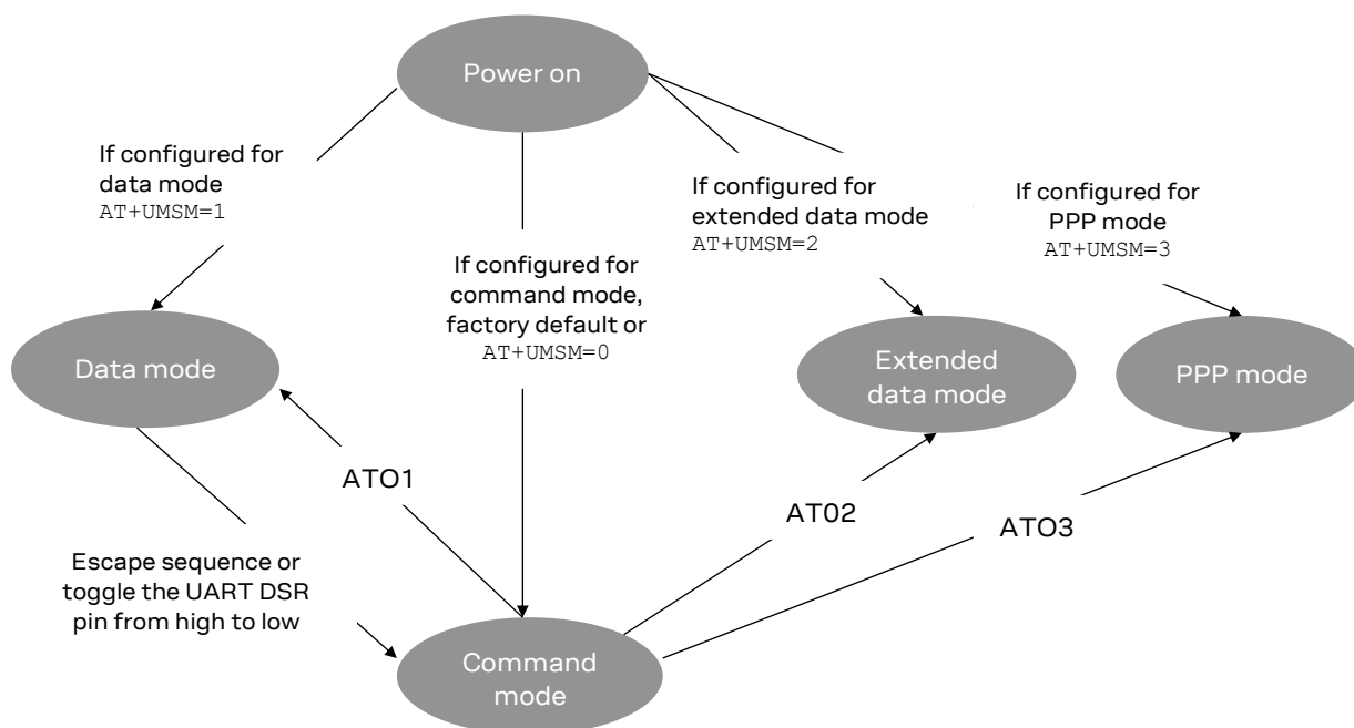
Figure 15: State diagram showing operational mode transitions
