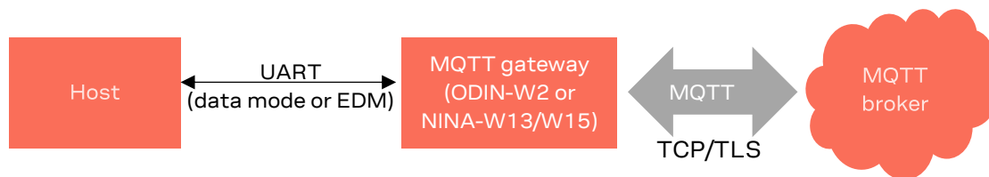
Figure 39: Host to MQTT broker communication
