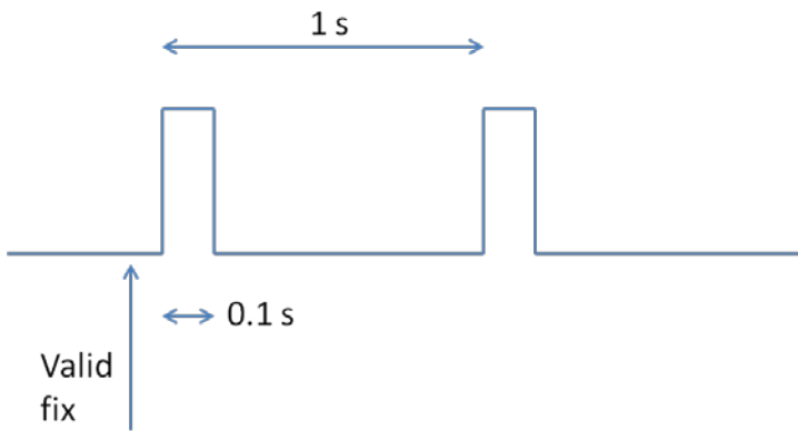
Figure 5: UI_FIX valid fix indicator timing
