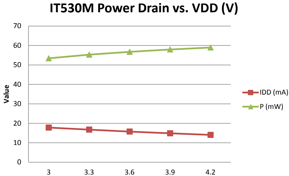
Figure 3: IT530M Power Drain (typ.) vs. VDD (V)
