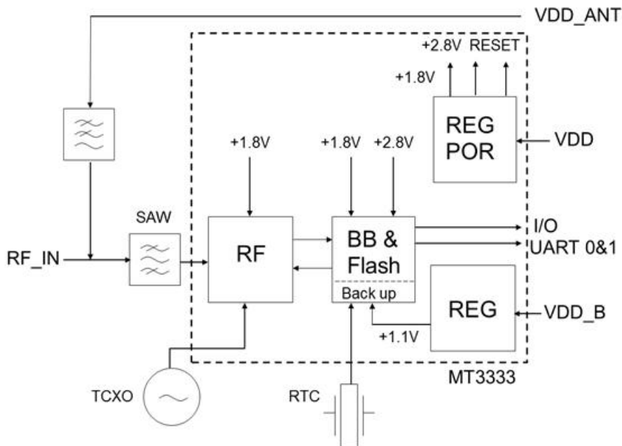
Figure 1: Block diagram
