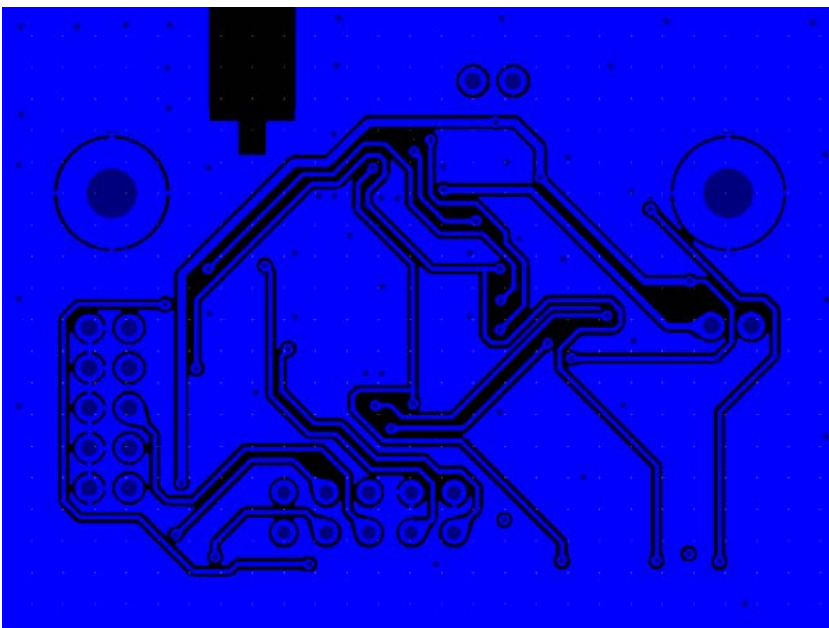
Figure 16: Layer 3
