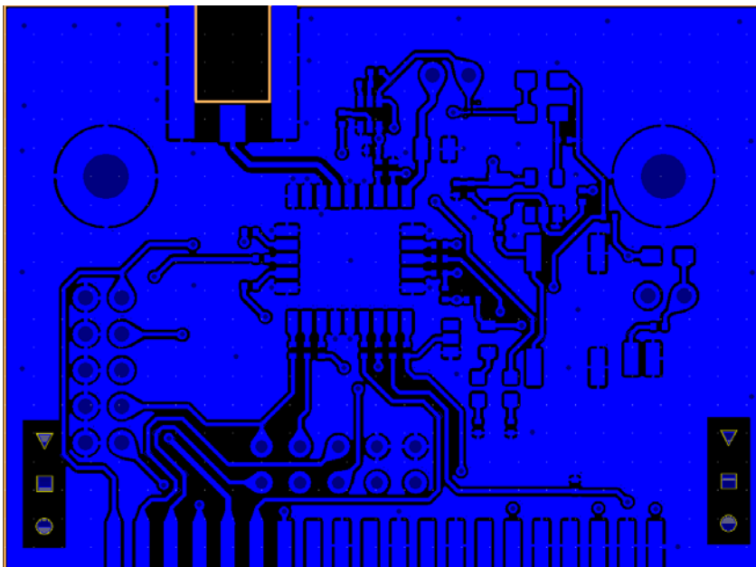
Figure 14: Layer 1, (top)
