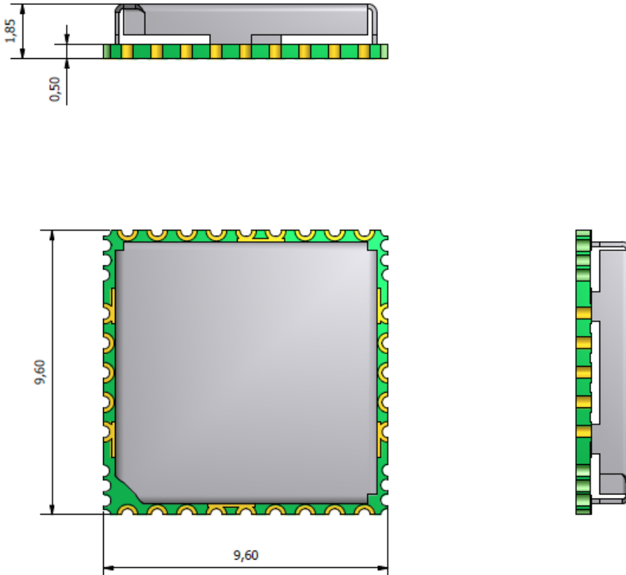
Figure 6: Mechanical dimensions
