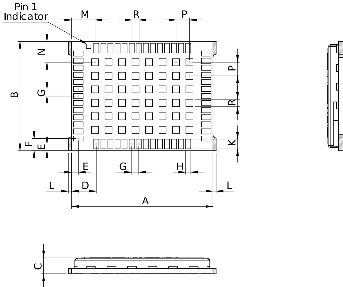
Figure 5: ZED-F20P mechanical drawing
