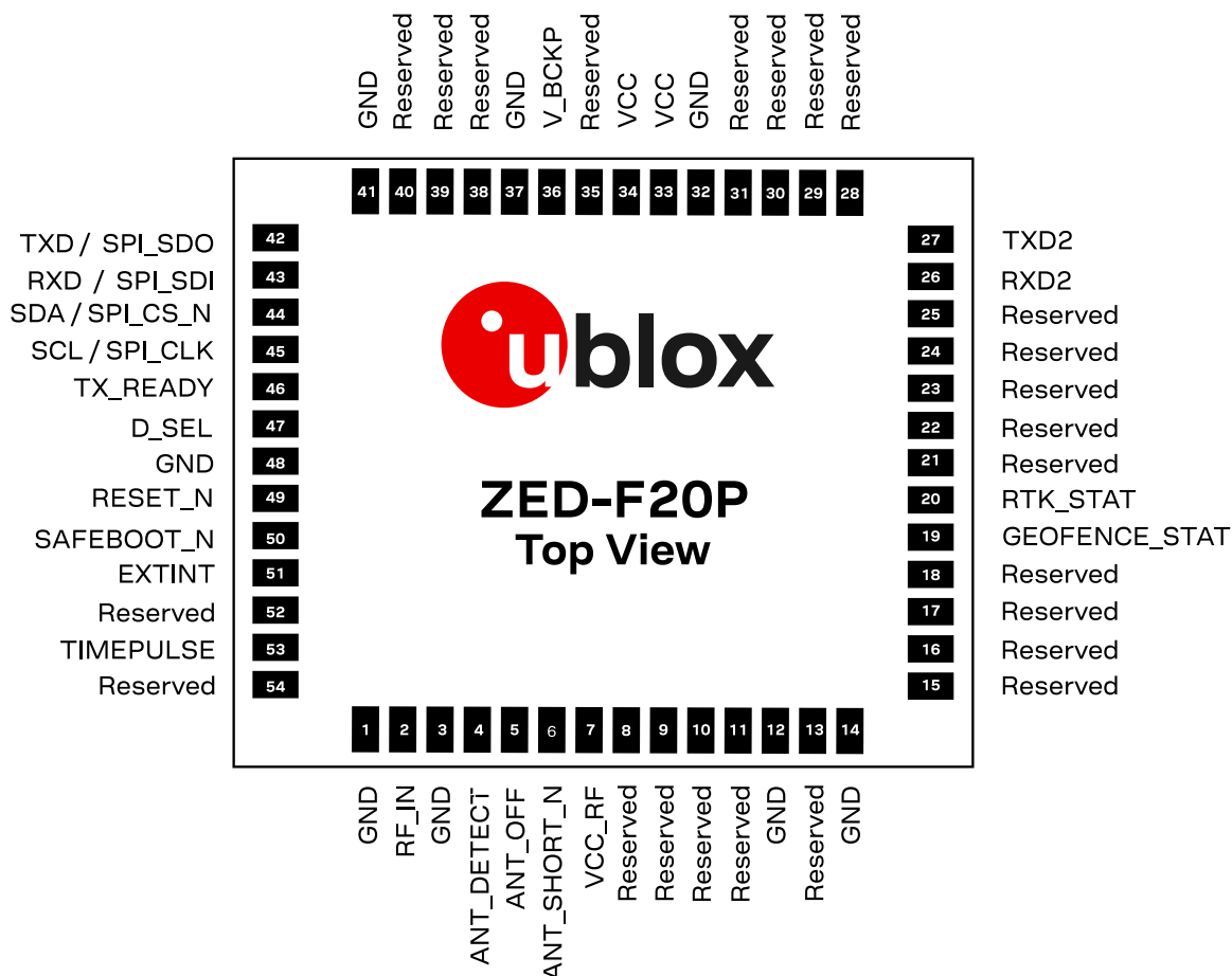
Figure 2: ZED-F20P pin assignment
