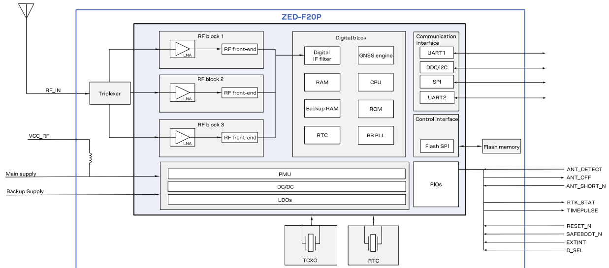
Figure 1: ZED-F20P block diagram
