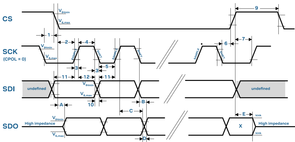
Figure 3: ZED-F20P SPI specification mode 1: CPHA=0 SCK = 5.33 MHz
