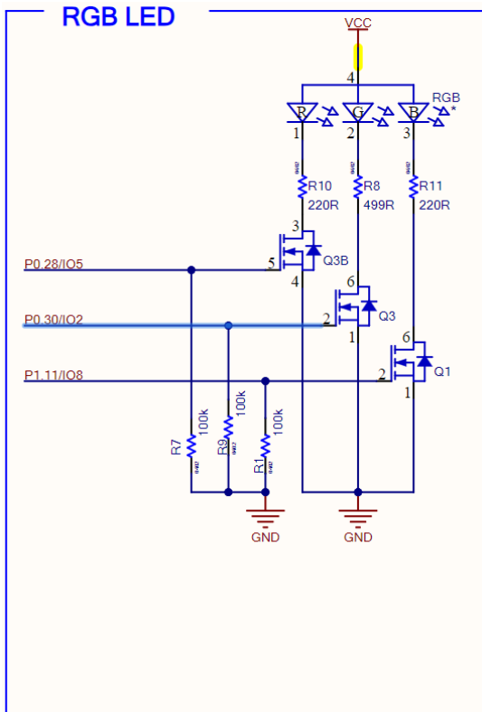
Figure 16: RGB LED circuit
