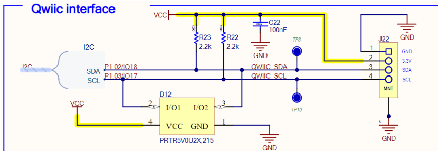
Figure 14: Qwiic connector
