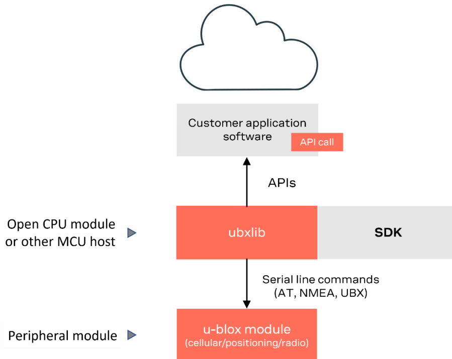
Figure 24: ubxlib MCU host and peripheral configuration
