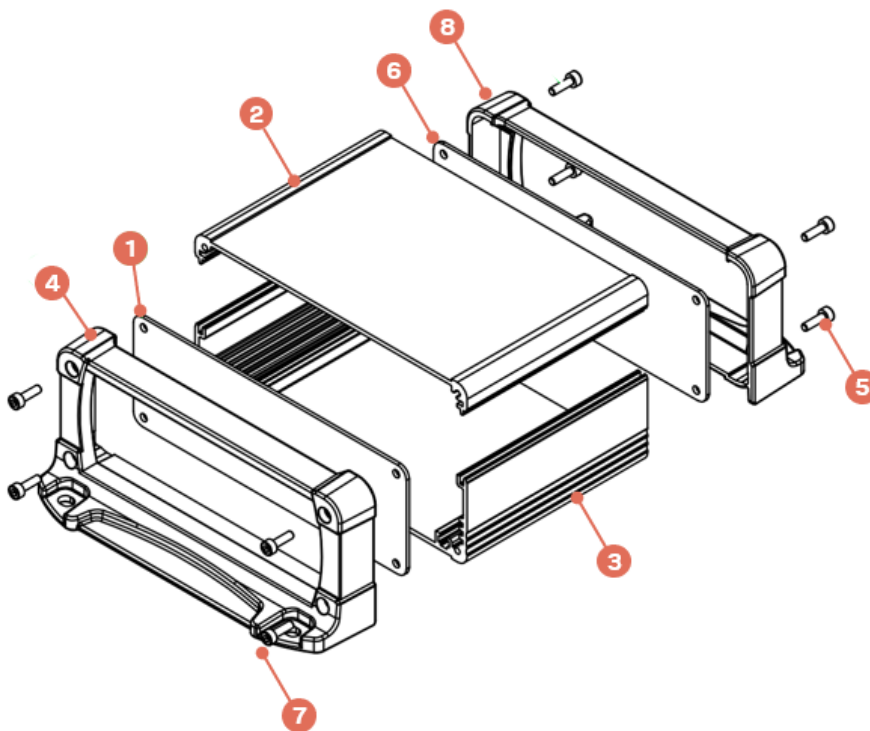
Figure 28: Enclosure parts
