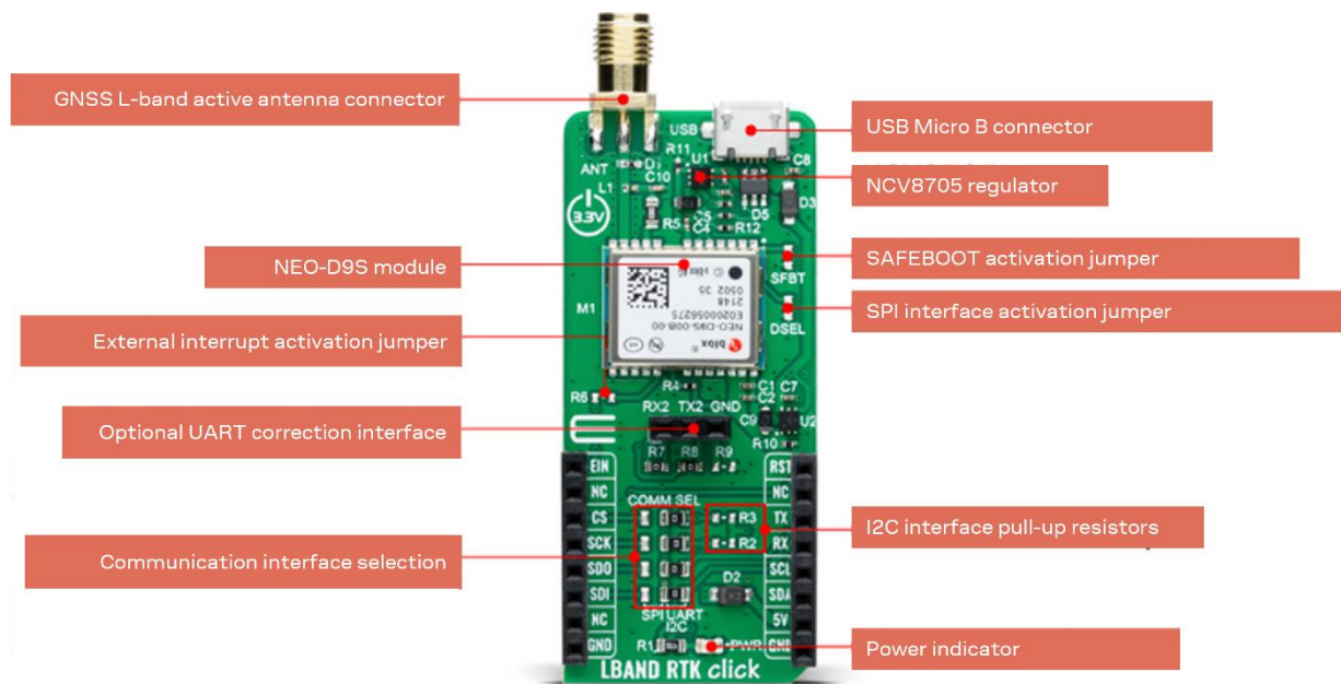
Figure 21: LBAND RTK Click board
