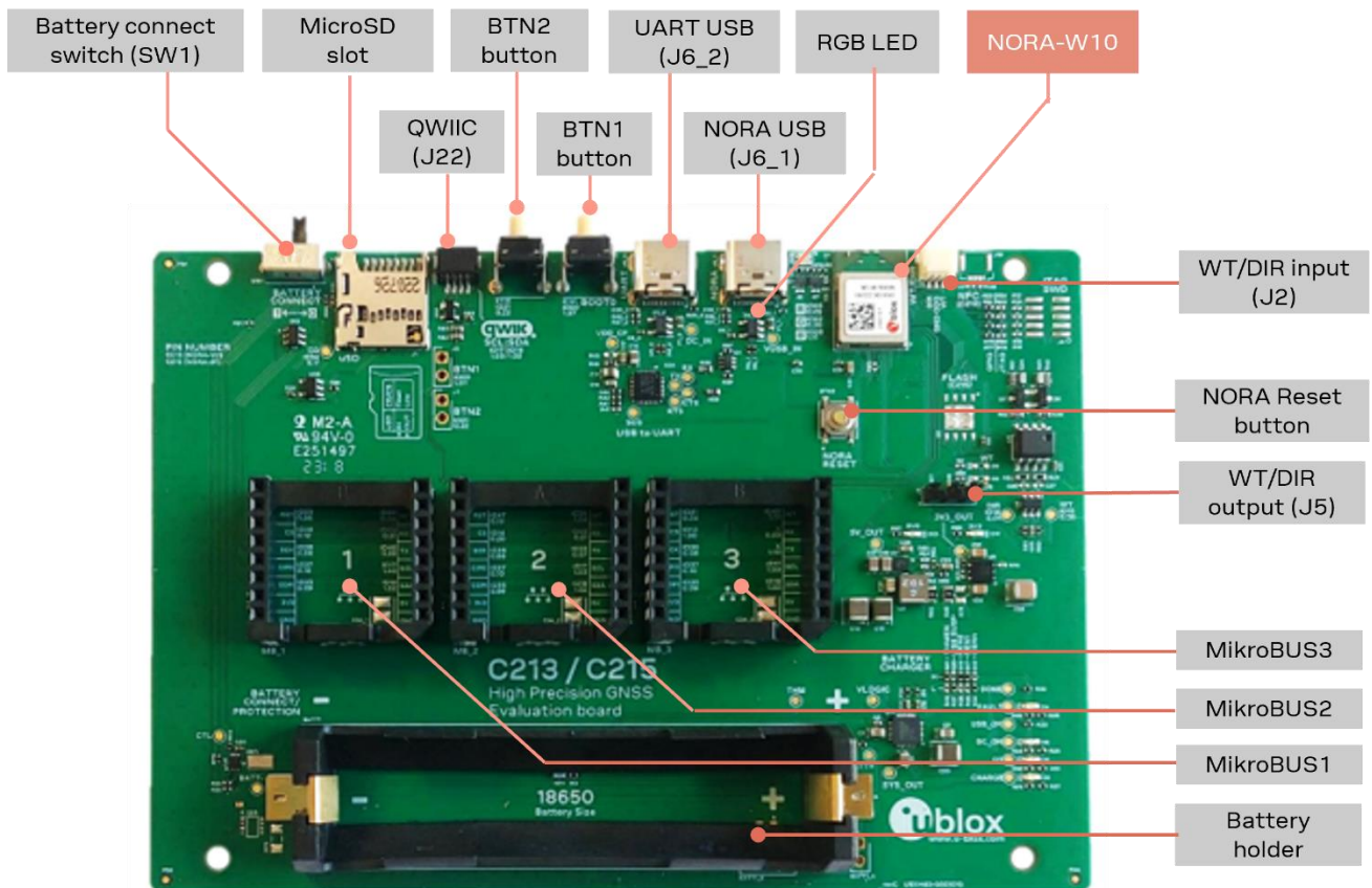
Figure 6: C213 baseboard assembly
