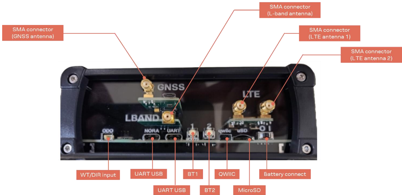
Figure 25: Kit enclosure showing access to antennas, buttons, switches, and connectors
