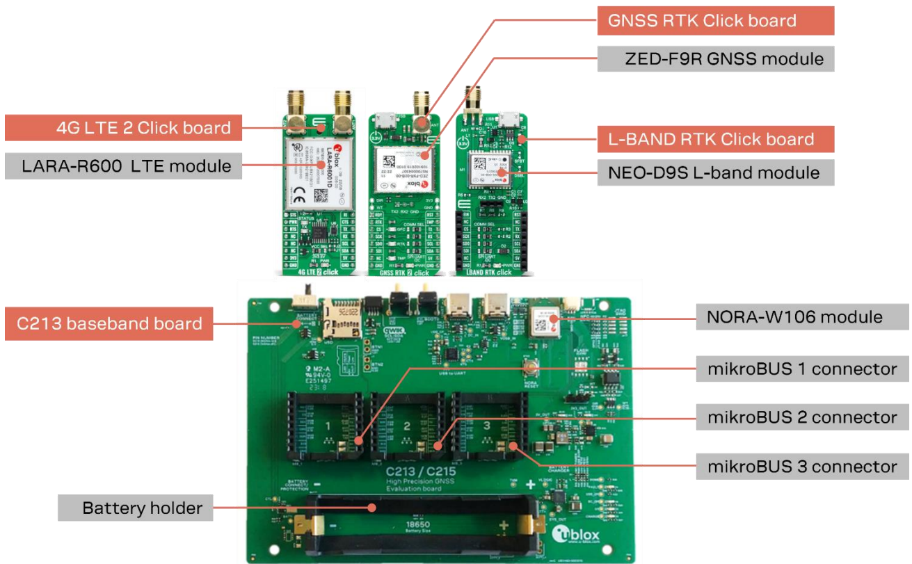
Figure 2: XPLR-HPG-1 board assemblies
