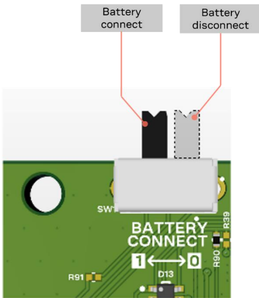
Figure 11: SW1 (battery connect switch) positions
