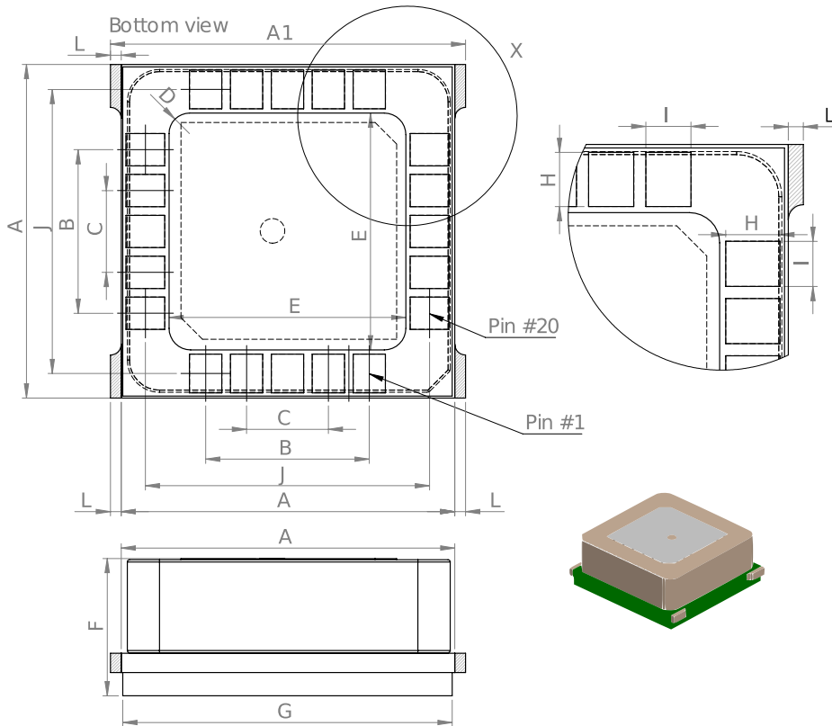
Figure 3 Dimensions
