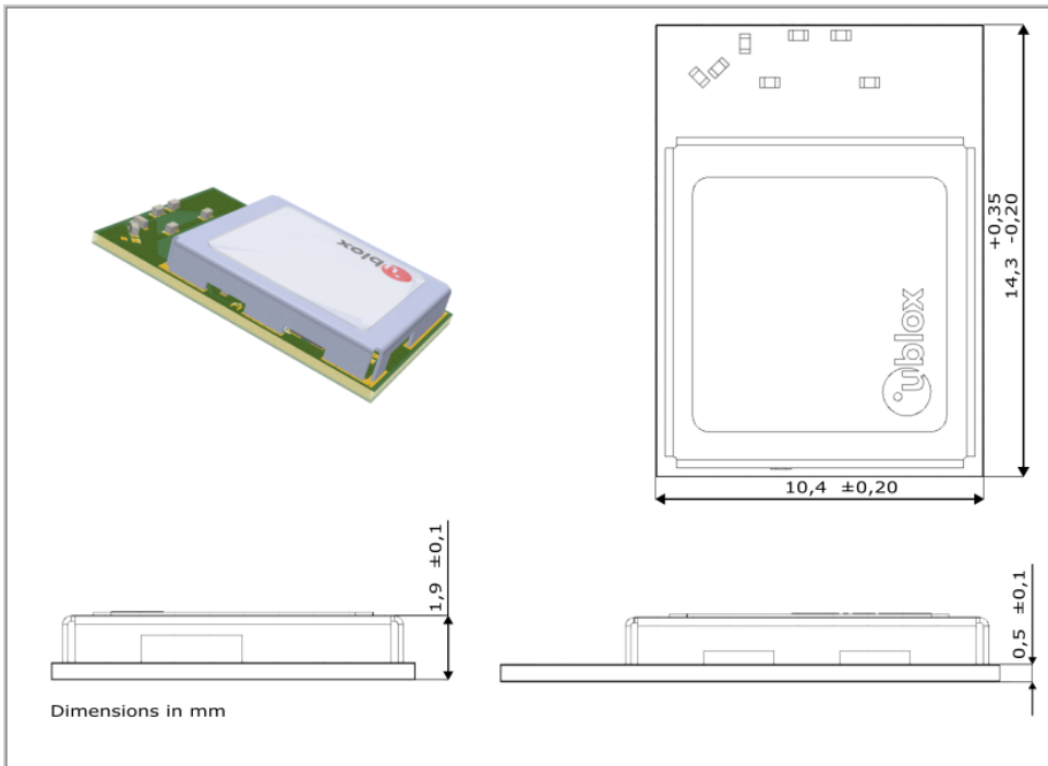
Figure 7: NORA-B2x6 mechanical specification
