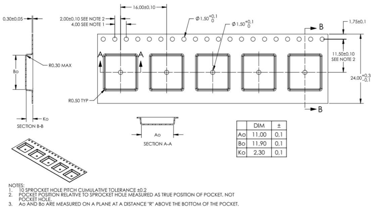
Figure 12: Tape and pocket dimensions for NORA-B2x1
