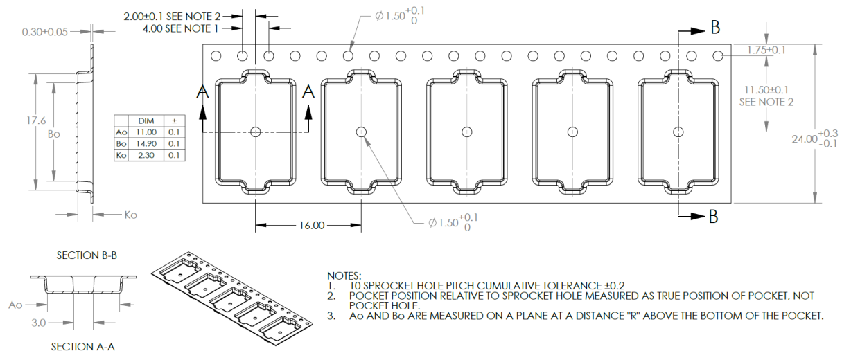
Figure 11: Tape and pocket dimensions for NORA-B2x6
