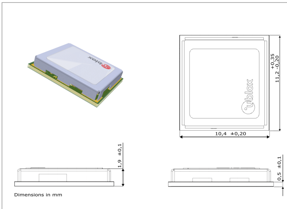
Figure 8: NORA-B2x1 mechanical specification
