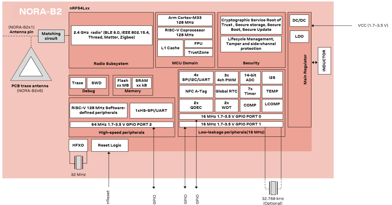
Figure 1: Block diagram of NORA-B2 series
