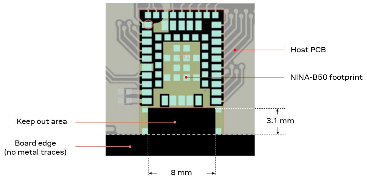
Figure 11: NINA-B506 keep out area
