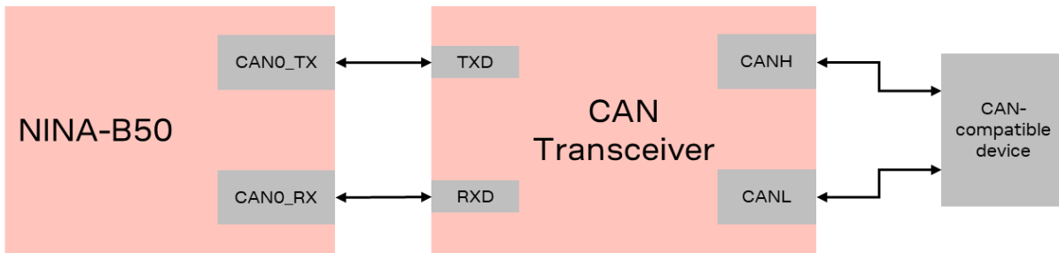
Figure 7: FlexCAN implementation
