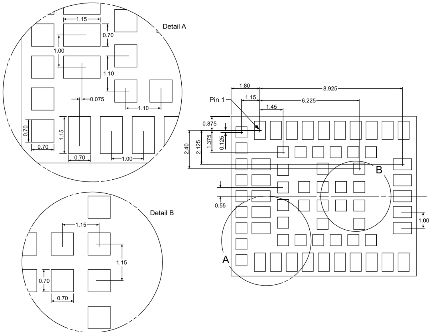
Figure 12: Recommended footprint for NINA-B501 (bottom view)
