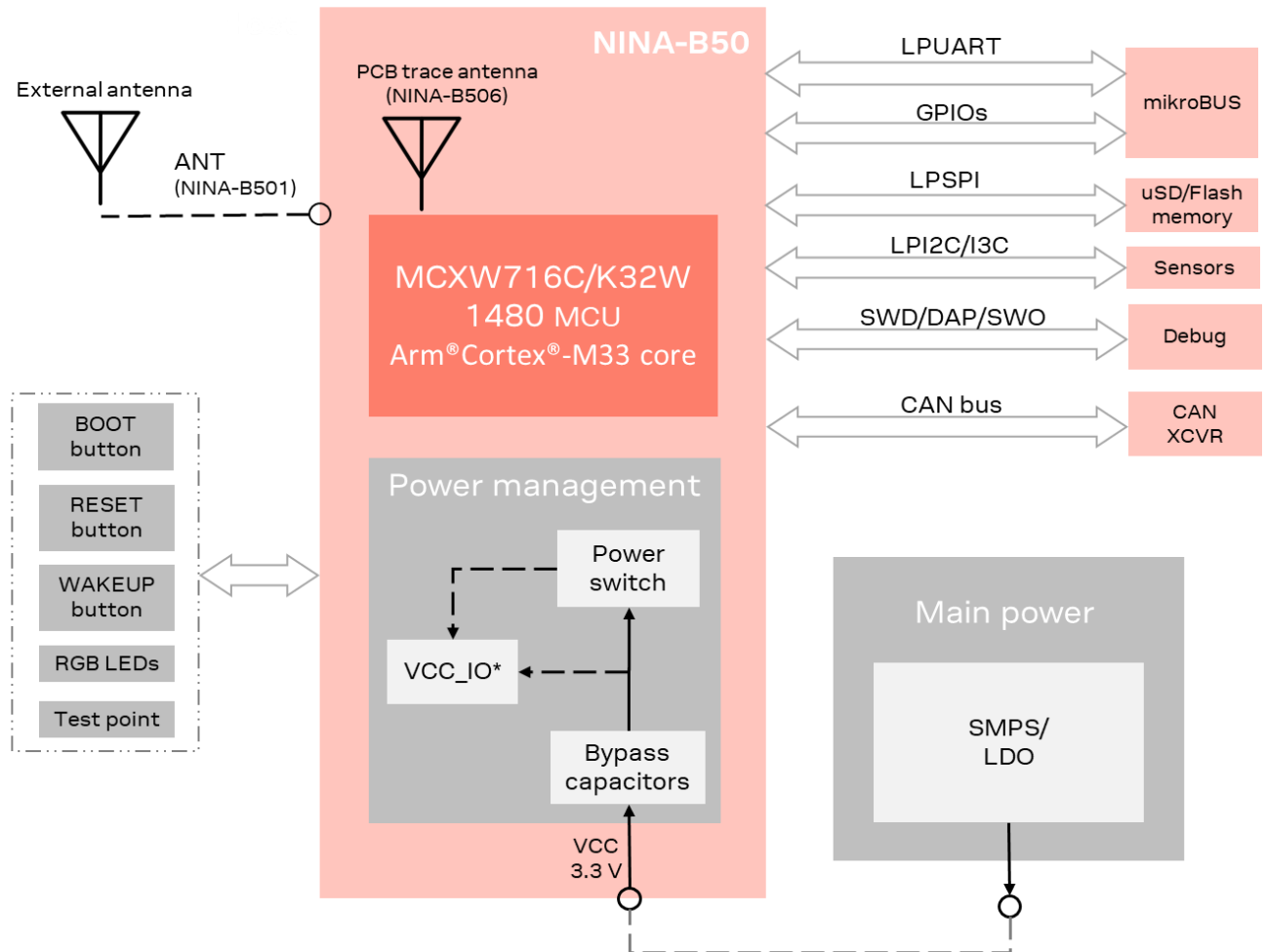
Figure 1: Example of NINA-B50 integrated as a host
