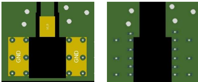
Figure 9: U.FL connector layout showing top layer (left) and inner layer 1 (right)
