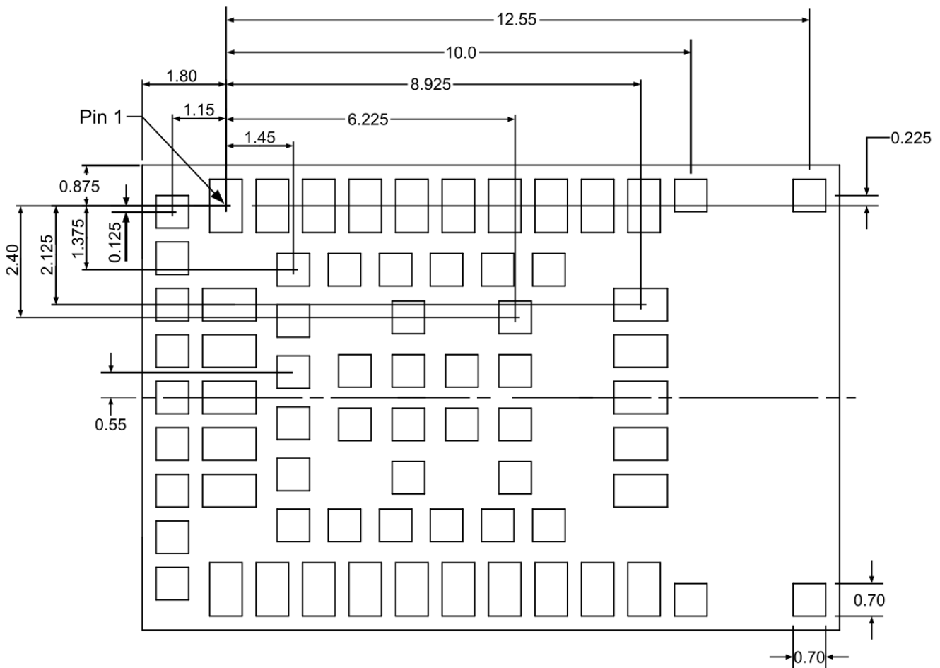
Figure 13: Recommended footprint for NINA-B506 (bottom view)
