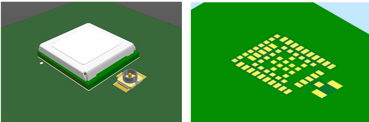
Figure 25: U.FL connector placement (left) and module footprint (right)
