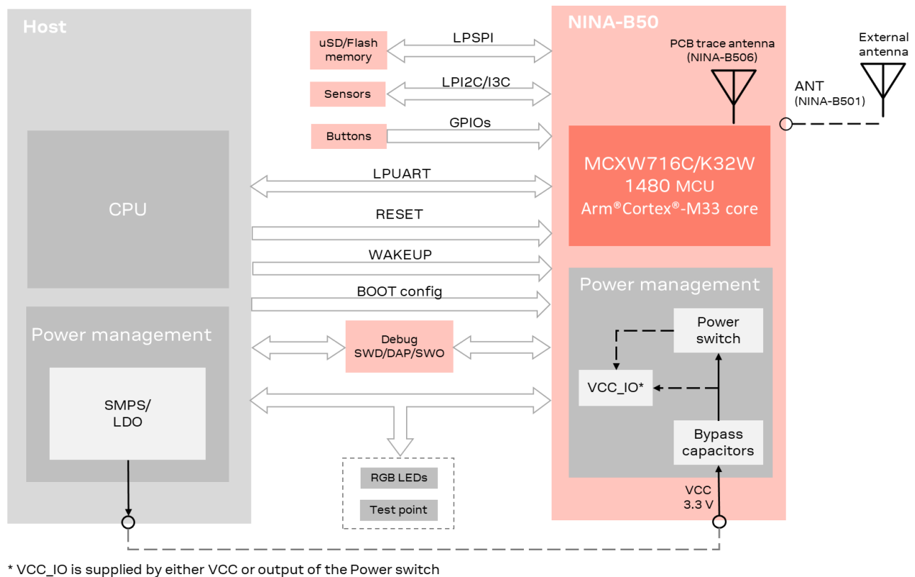
Figure 2: Example of NINA-B50 integration in a host system with external CPU
