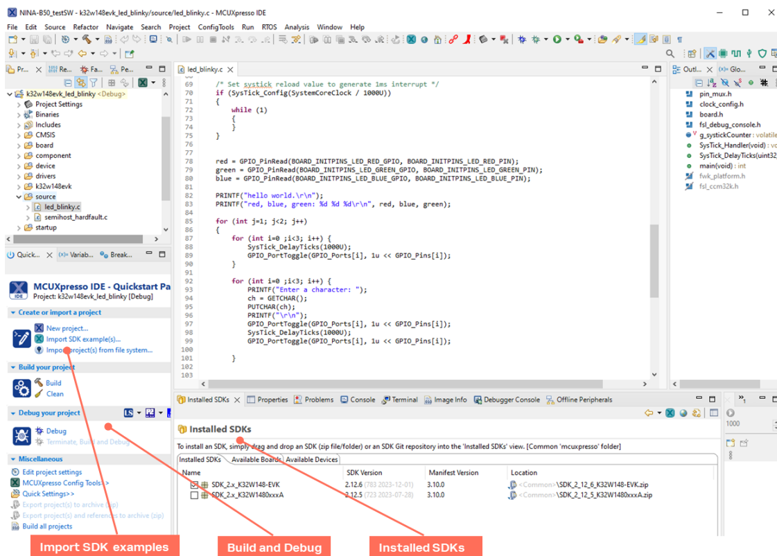
Figure 14: Installed SDKs
