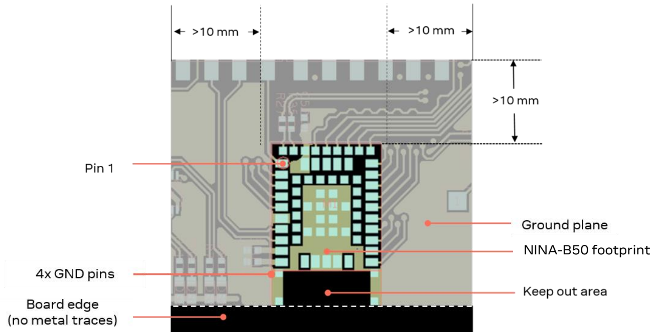
Figure 10: Extended host ground plane outside NINA-B506
