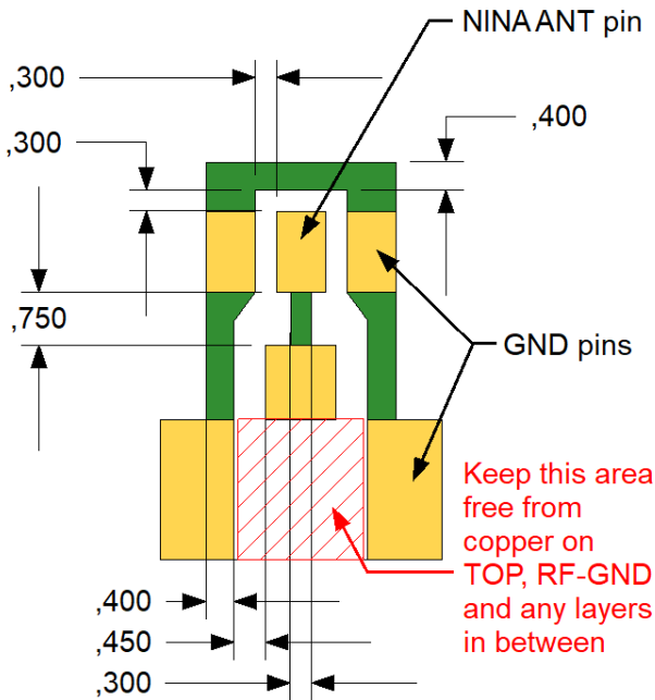
Figure 28: RF trace and minimum required GND trace of the U.FL antenna connector reference design
