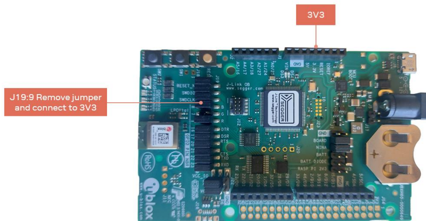
Figure 17: EVK-NINA-B5 jumper settings and wiring for entering bootloader mode
