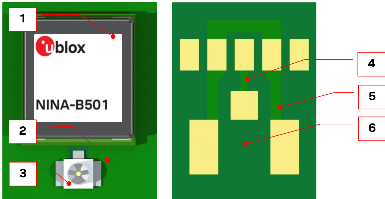
Figure 26: NINA-B501 antenna reference design
