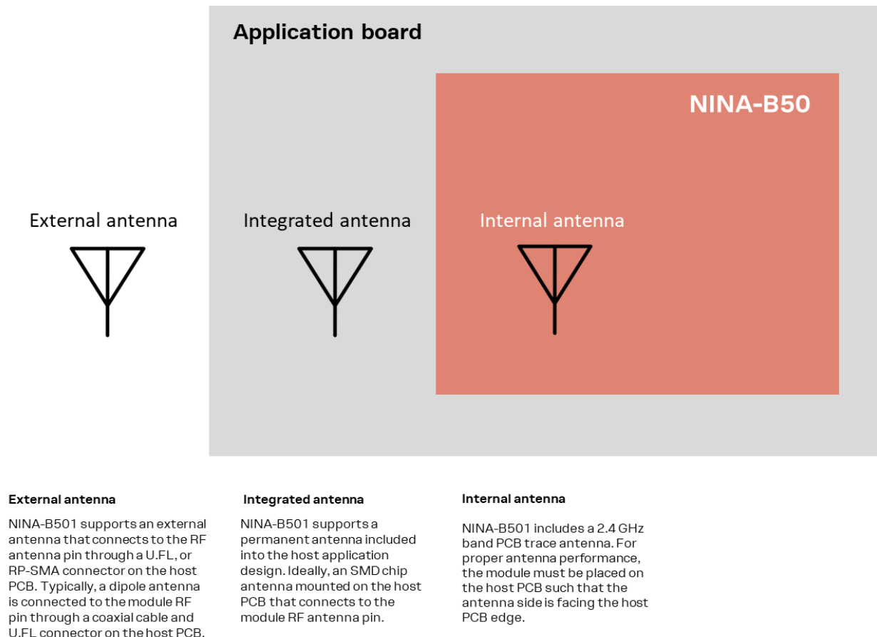
Figure 6: Antenna options
