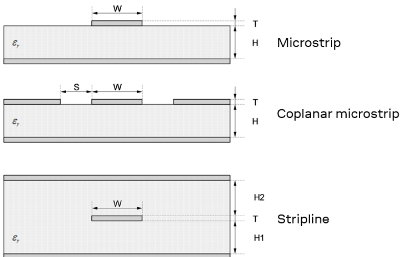
Figure 8: Transmission line trace design
