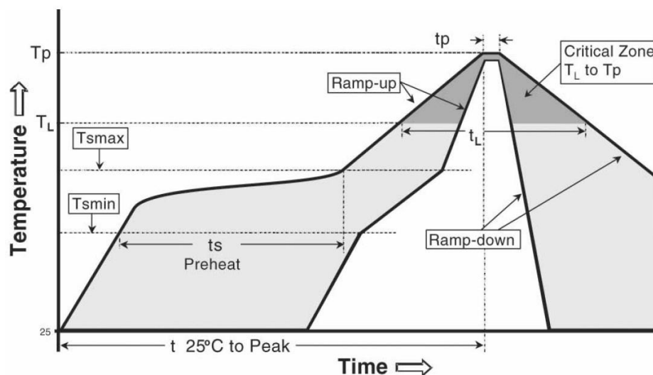
Figure 19: Reflow profile
