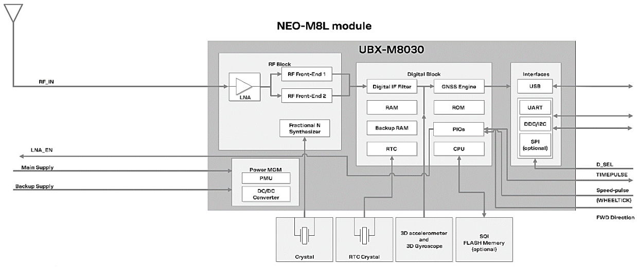
Figure 2: NEO-M8L-05B block diagram
