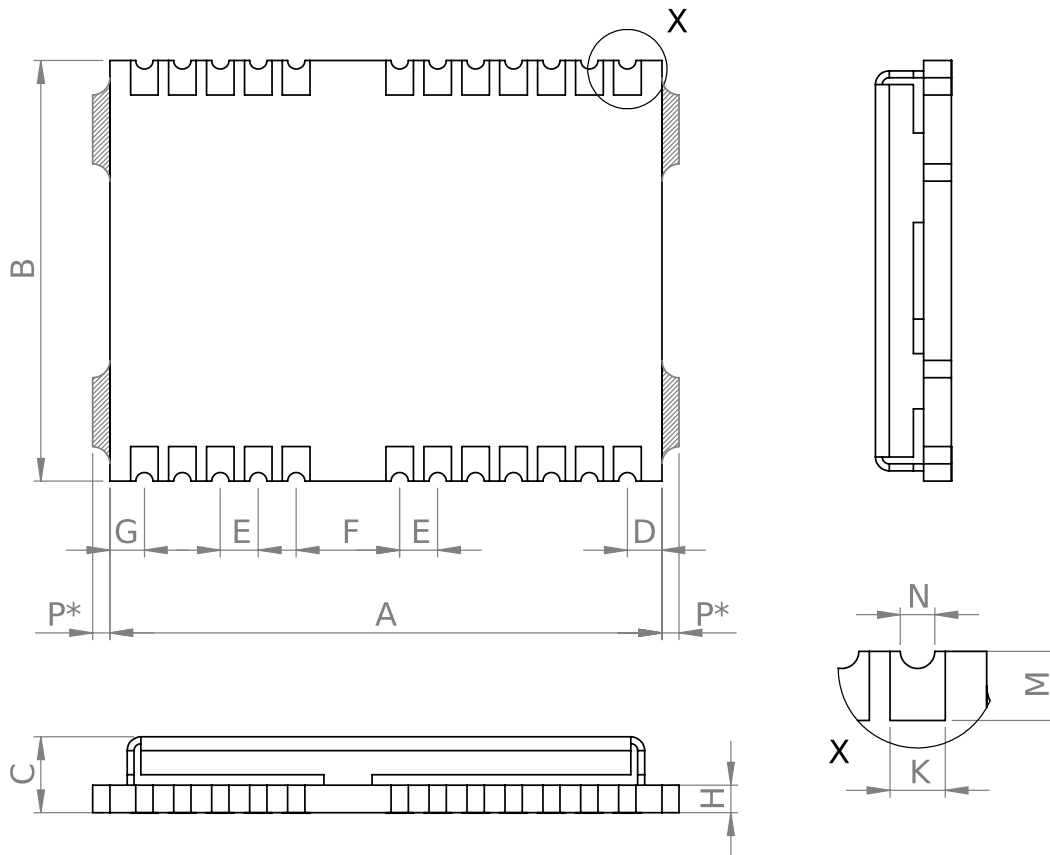
Figure 16 NEO-M8L-05B mechanical drawing
