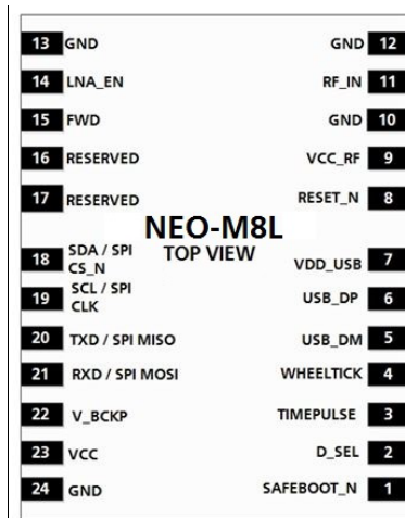
Figure 7: Pin assignment
