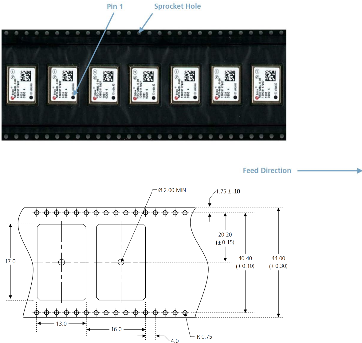
Figure 17: Dimensions and orientation for NEO-M8L-05B modules on tape
