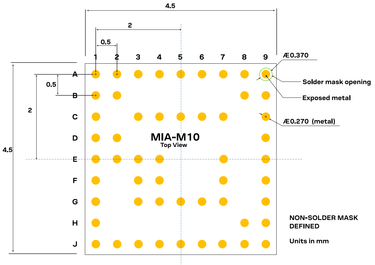
Figure 33: Recommended copper land and solder mask opening for MIA-M10C
