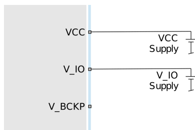
Figure 23: VCC and V_IO supplied by separate supplies. No external power supply at V_BCKP.
