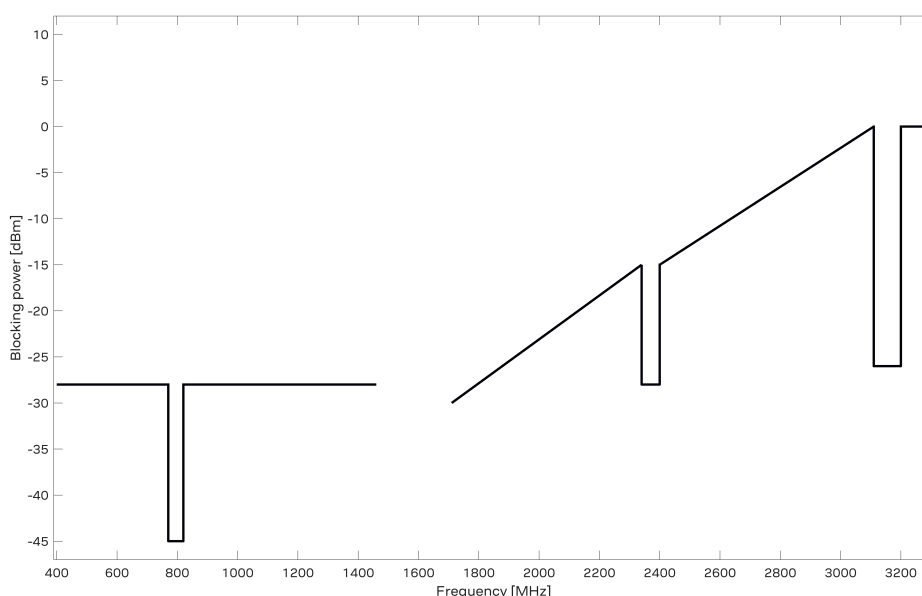
Figure 28: MIA-M10C out-of-band immunity level at 400–1460 MHz and 1710–3300 MHz for the normal-gain mode (default). Preliminary data subject to change.
