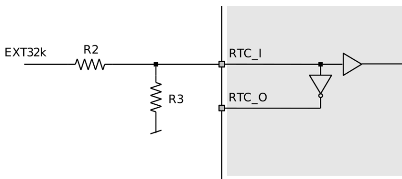
Figure 25: An external RTC signal
