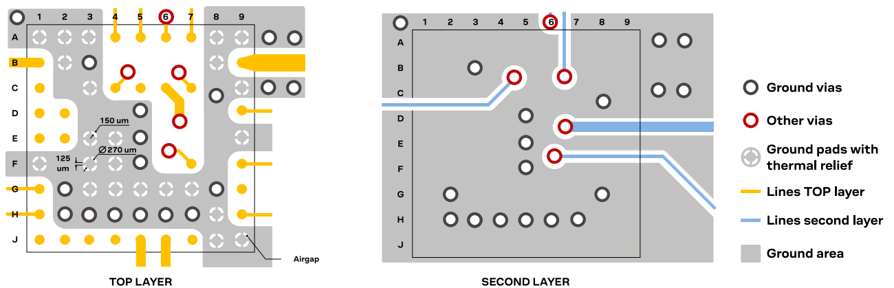
Figure 31: Example of a 2-layer design for MIA-M10C
