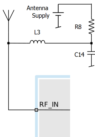
Figure 29: Antenna supply network
