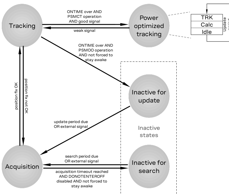
Figure 12: State machine
