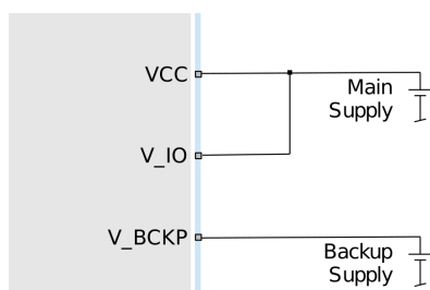
Figure 20: VCC and V_IO connected to the main supply, and external power supply at V_BCKP
