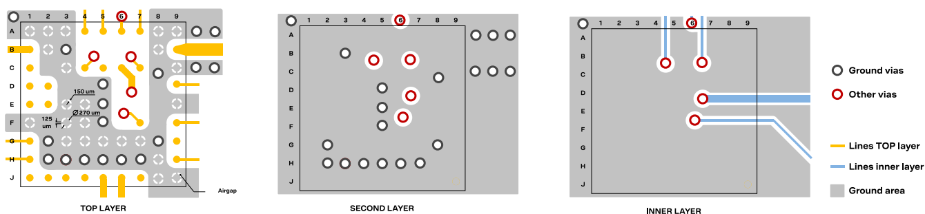
Figure 32: Example of a +2 layer design for MIA-M10C
