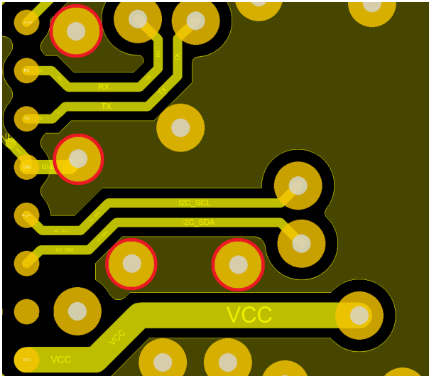
Figure 30: GND stub ended with a via highlighted in red
