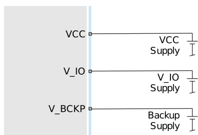
Figure 22: VCC and V_IO supplied by separate supplies, and external power supply at V_BCKP
