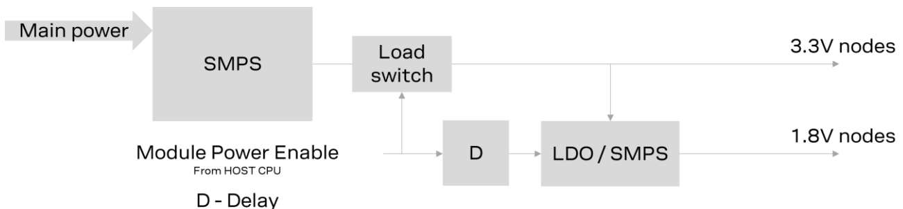
Figure 2: Proposed implementation of MAYA-W4 power supply circuitry
