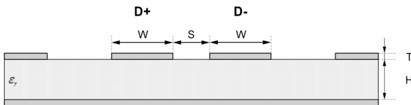
Figure 13: USB differential pair showing key parameters for controlled impedance
