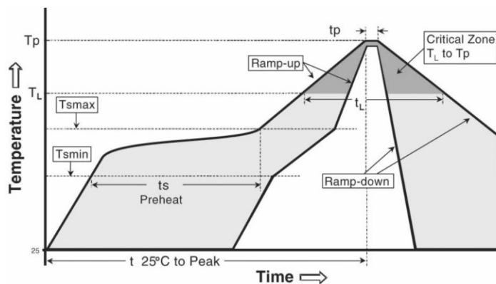
Figure 17: Reflow profile
