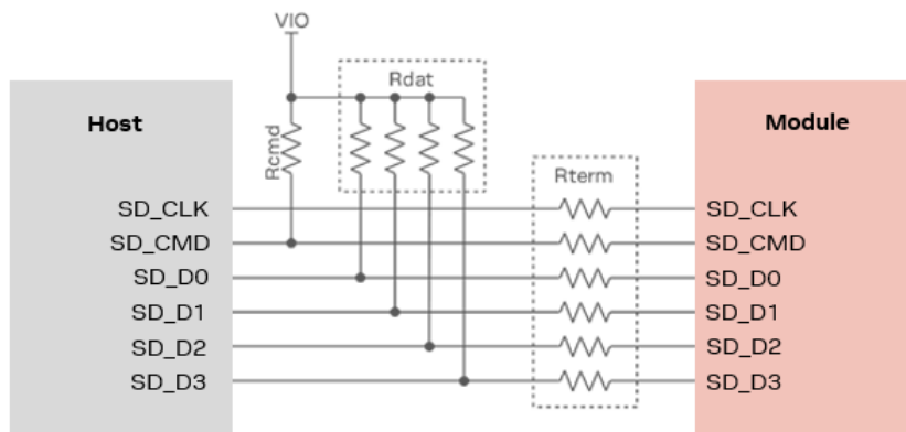
Figure 12: SDIO application schematic
