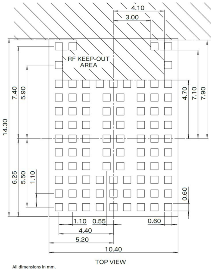
Figure 14: Recommended footprint for MAYA-W4, bottom view
