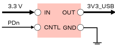
Figure 7: Load switch implementation using a dedicated IC
