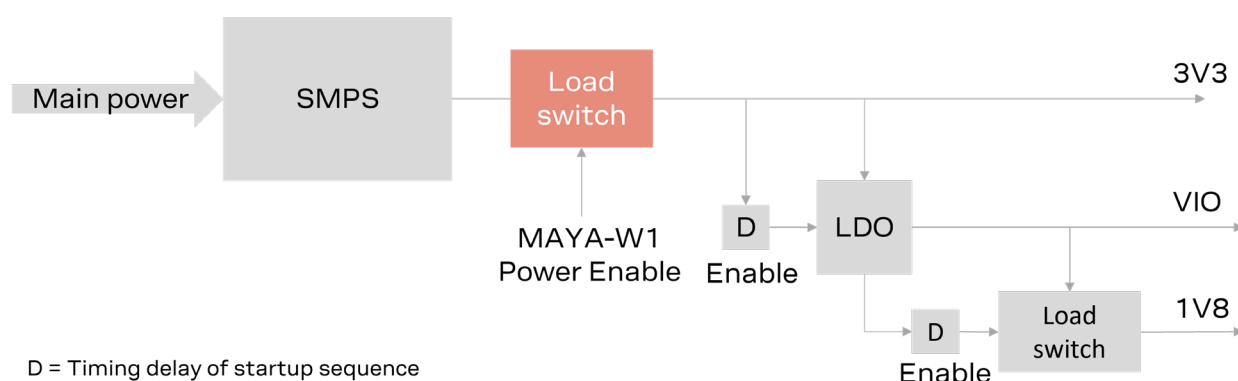
Figure 4. Example of hardware-sequenced power supply
