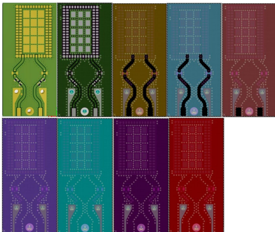
Figure 10: RF trace and ground design example
