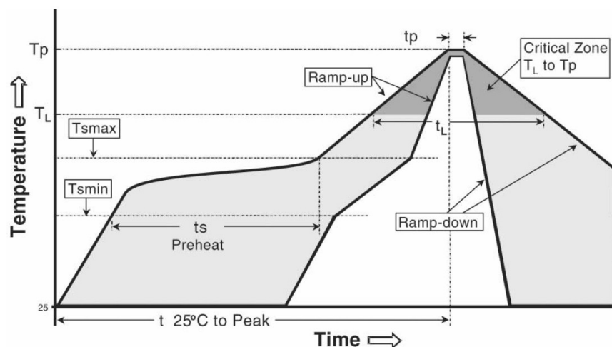
Figure 17: Reflow profile
