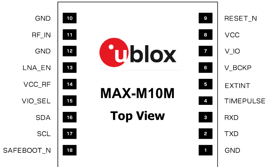
Figure 2: MAX-M10M-00B pin assignment
