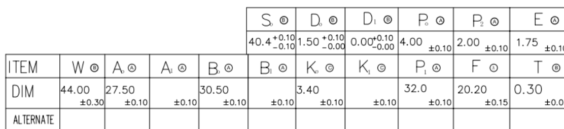
Figure 8: LENA-R8 series modules tape dimensions
