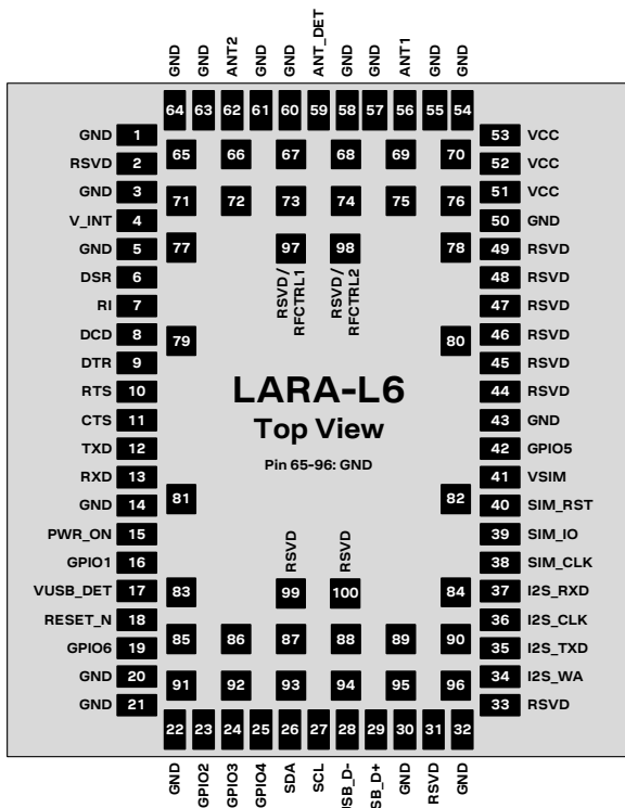
Figure 2: LARA-L6 series pin assignment (top view)
