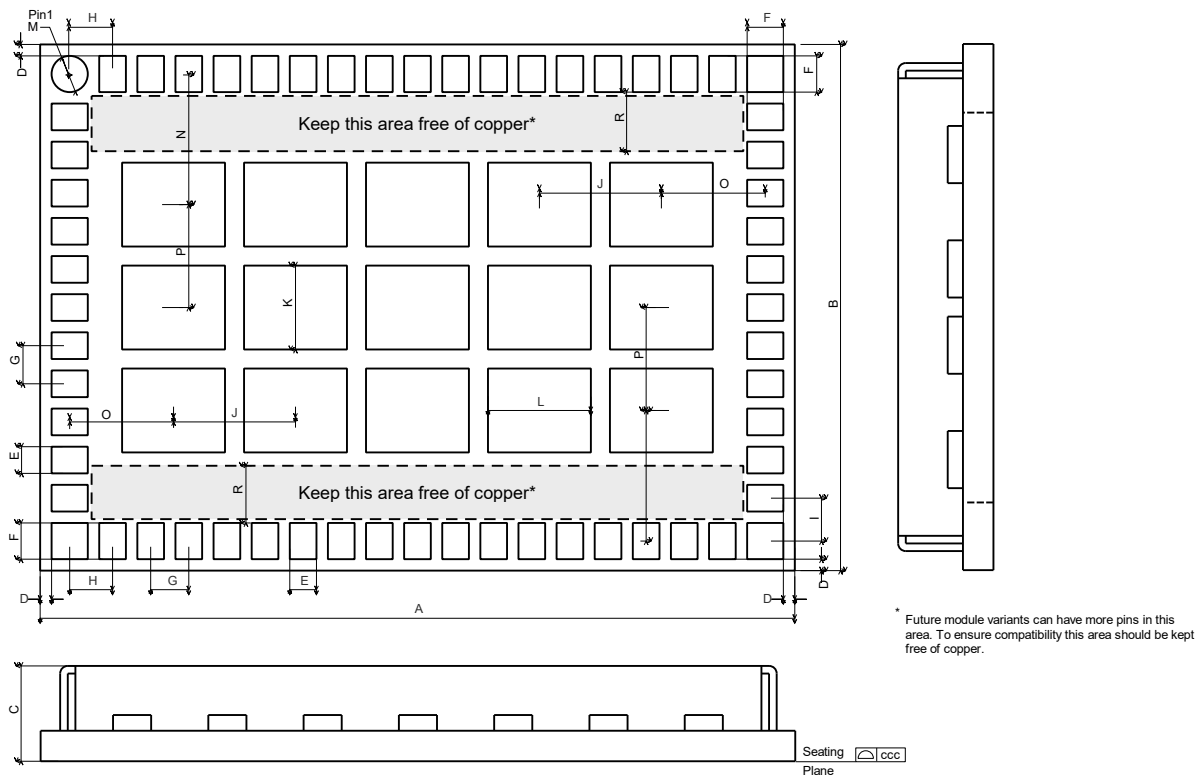
Figure 12: JODY-W2 series dimensions (bottom view)
