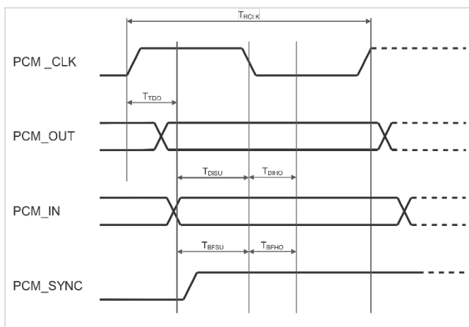
Figure 10: PCM timing specification – Peripheral mode
