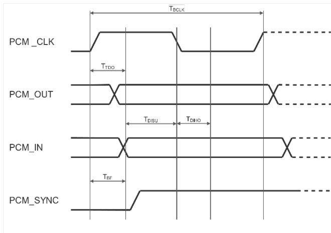
Figure 9: PCM timing specification – Central mode
