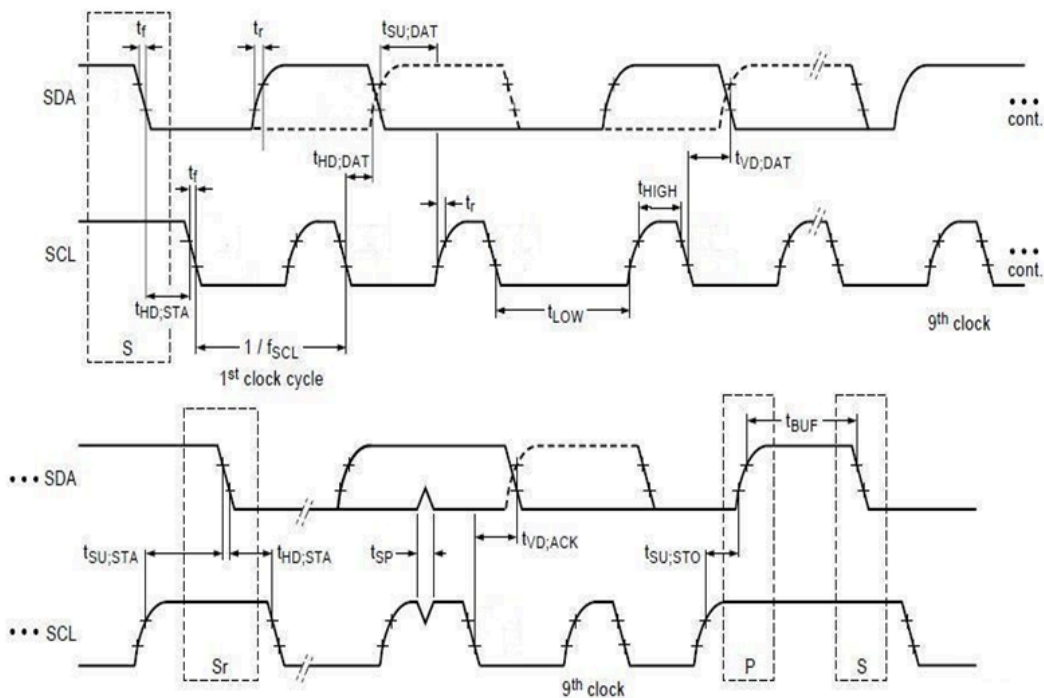
Figure 4: ZED-F9R-02B I2C peripheral specification
