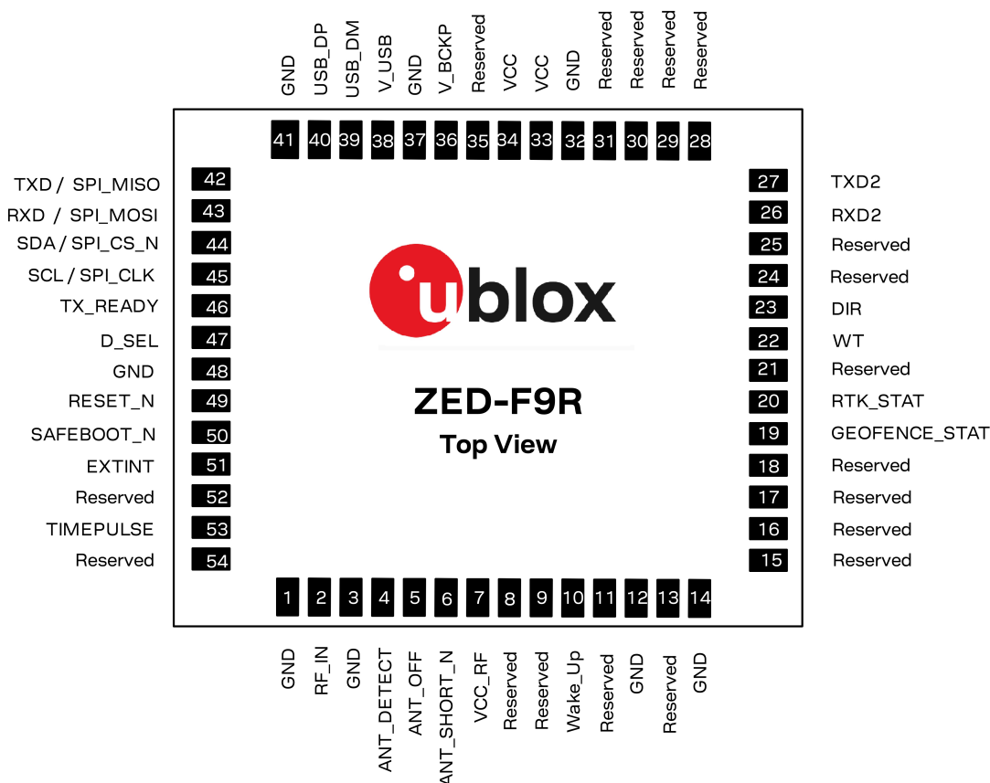
Figure 2: ZED-F9R-02B pin assignment
