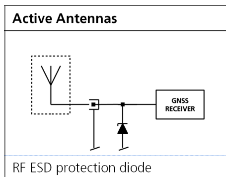
Figure 47: RF ESD precautions
