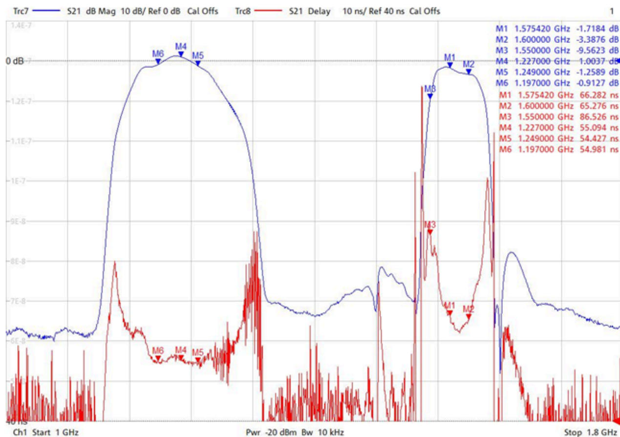
Figure 71: Low-cost L1/L2 antenna band characteristics
