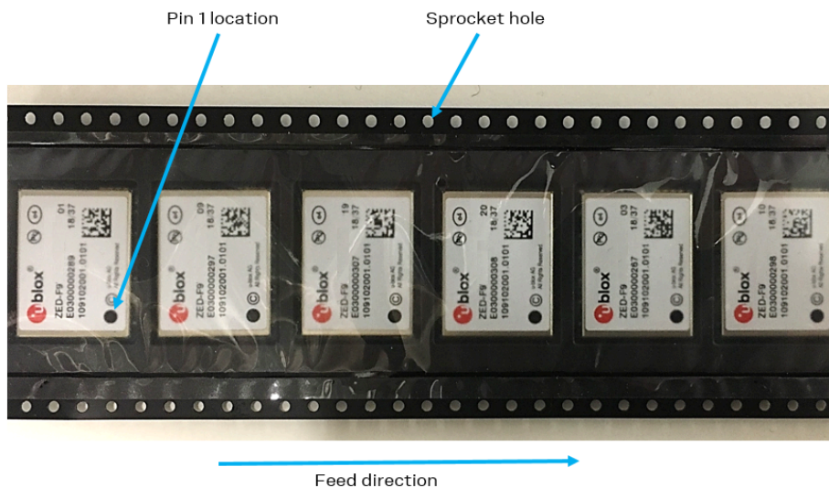
Figure 57: Orientation of ZED-F9P on the tape
