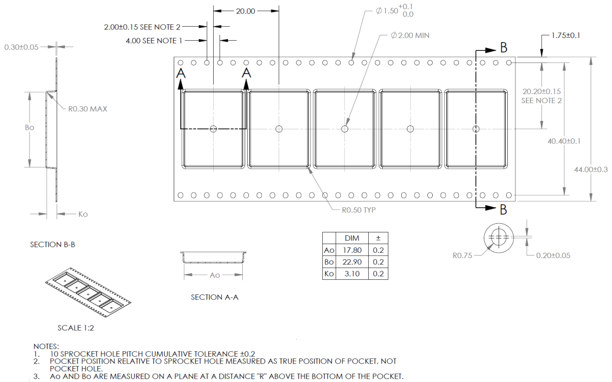
Figure 58: ZED-F9P tape dimensions (mm)
