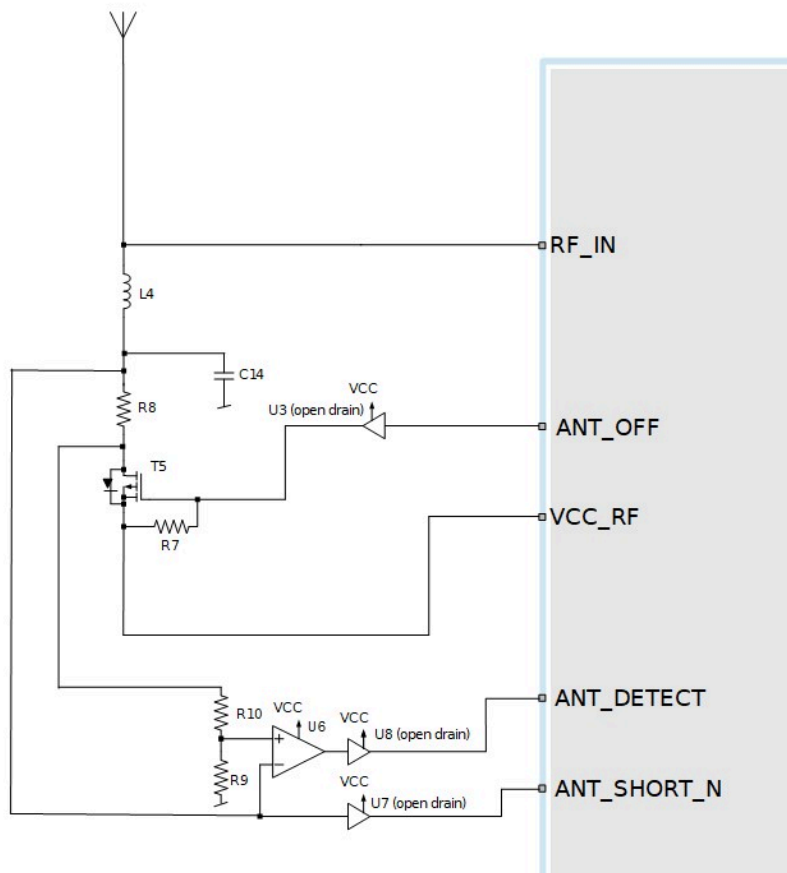
Figure 46: ZED-F9P antenna supervisor circuit
