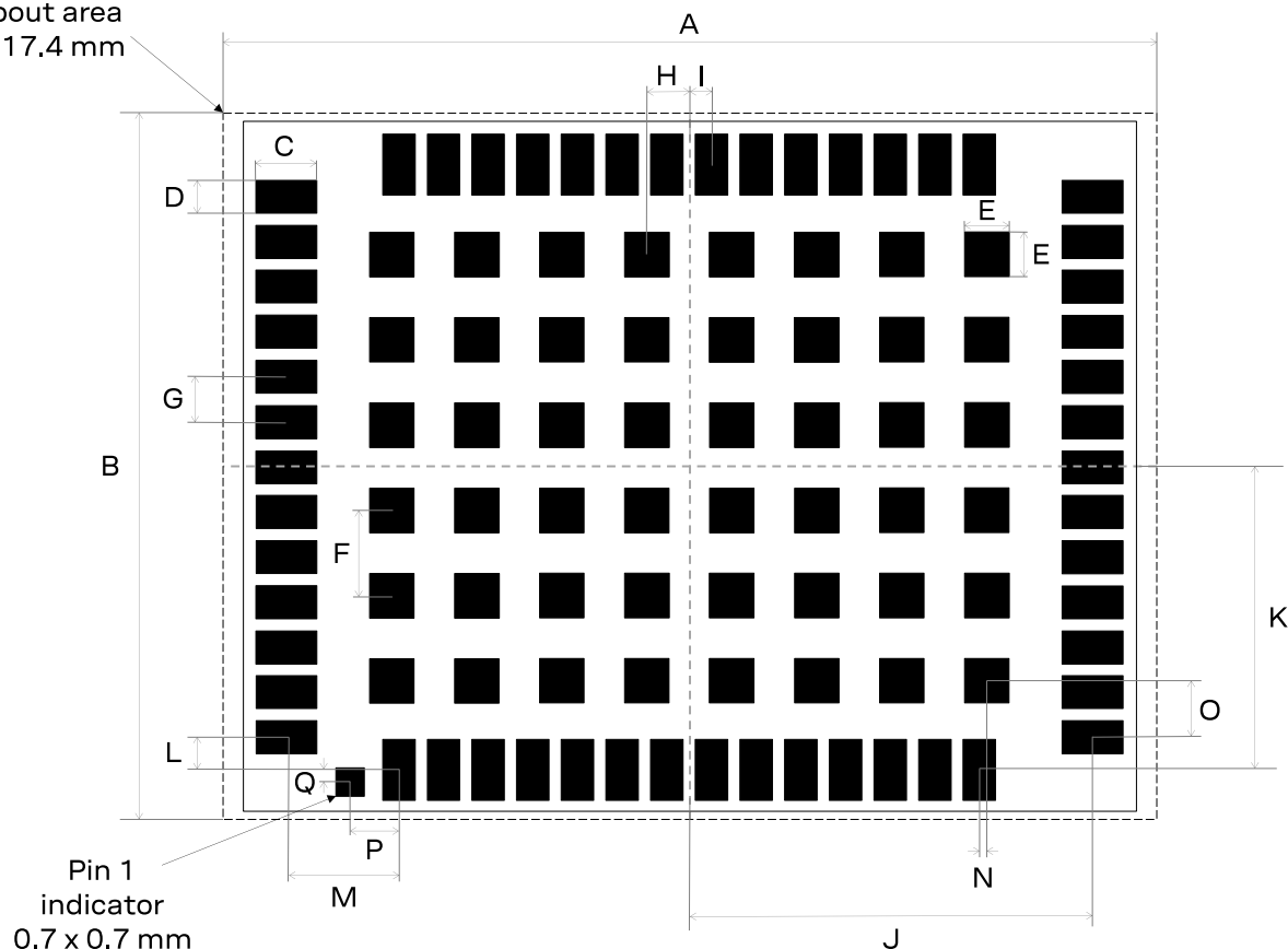
Figure 49: ZED-F9P suggested footprint (i.e. copper mask)
