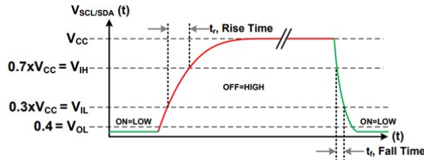
Figure 54: I2C bus signal rise and fall time
