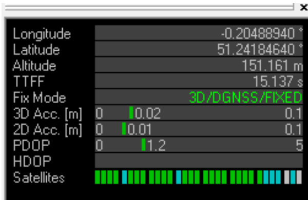
Figure 68: Rover: u-center data view with RTK Fixed
