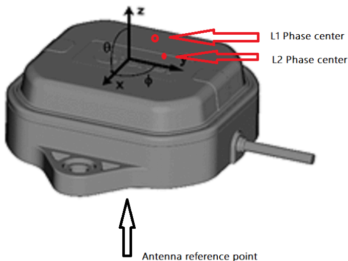
Figure 69: Stacked patch antenna
