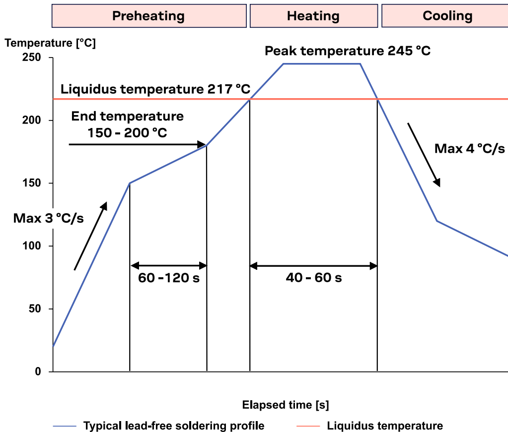
Figure 56: Recommended soldering profile for professional grade ZED-F9P
