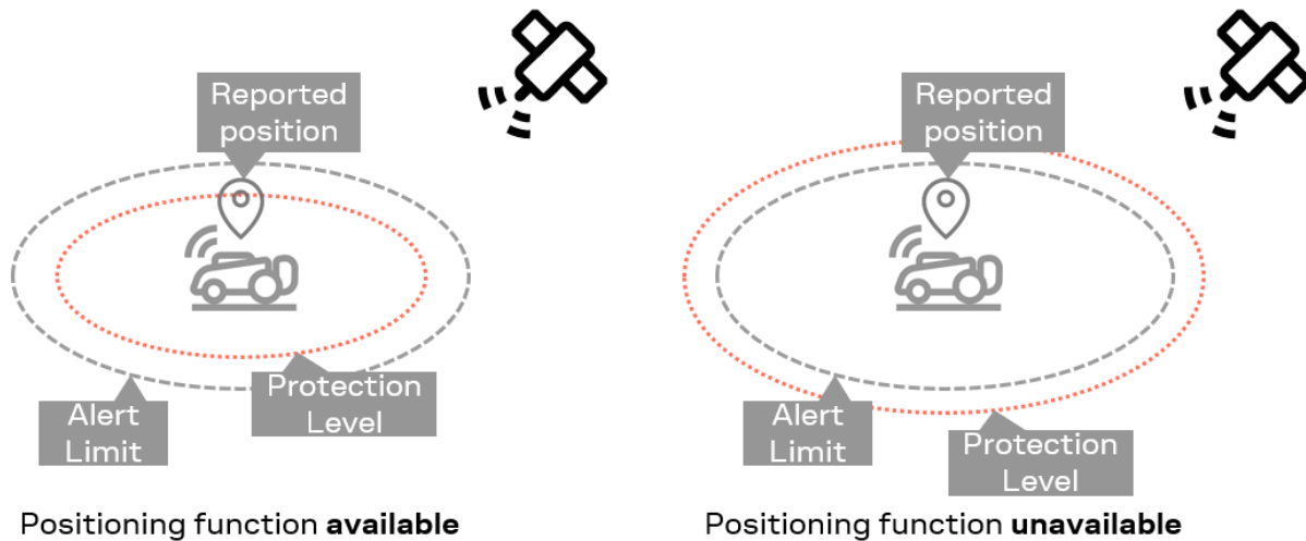
Figure 15: Positioning function
