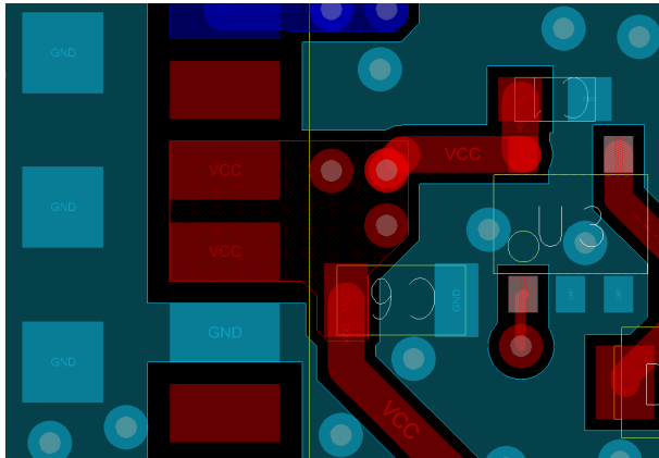
Figure 53: VCC pads
