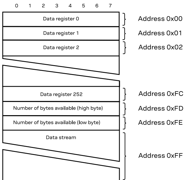
Figure 18: I2C register layout
