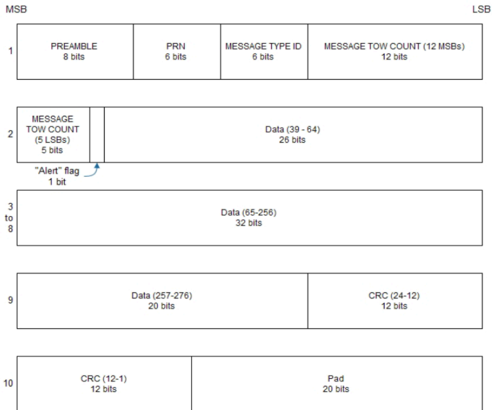
Figure 30: GPS L5 subframe words
