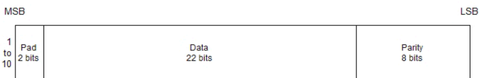
Figure 32: BeiDou subframe word
