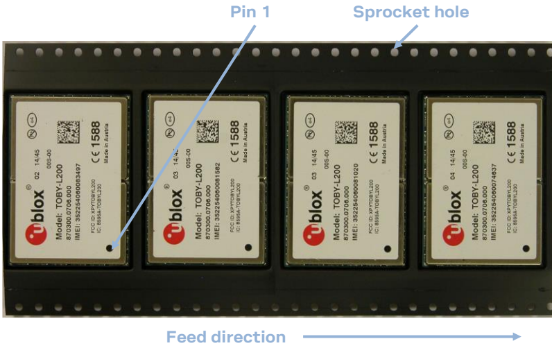
Figure 5: Orientation for TOBY-L2 modules on tape
