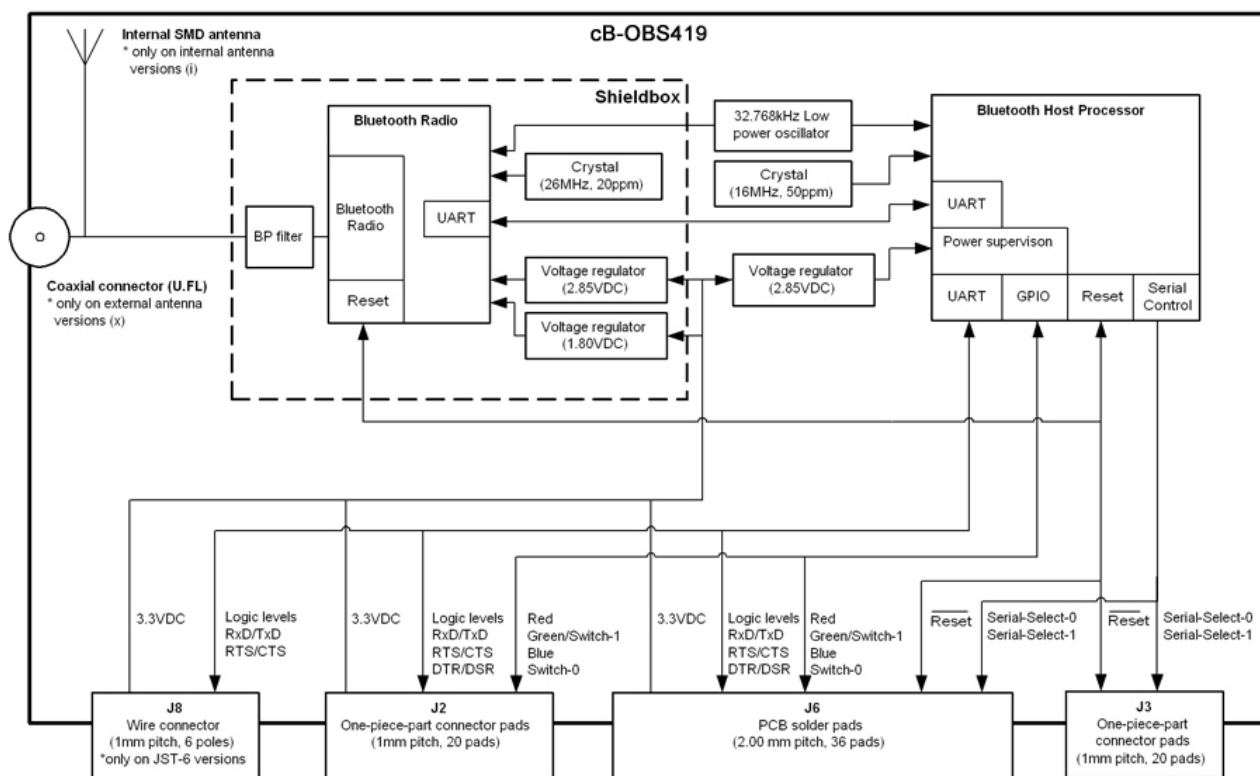
Figure 2: Block diagram of cB-OBS419
