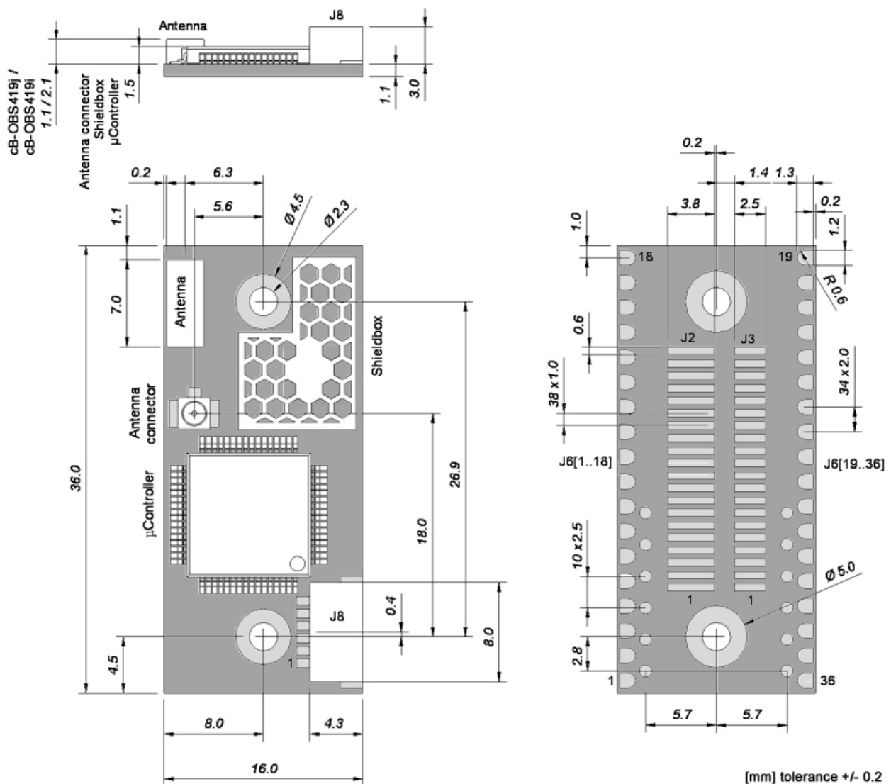
Figure 7: cB-OBS419 dimensions [mm].
