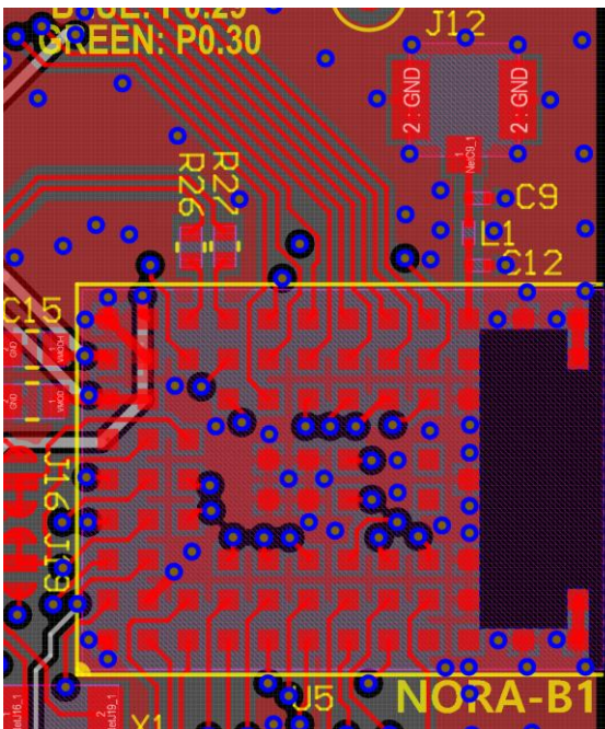
Figure 10: Example of RF trace and ground plane design
