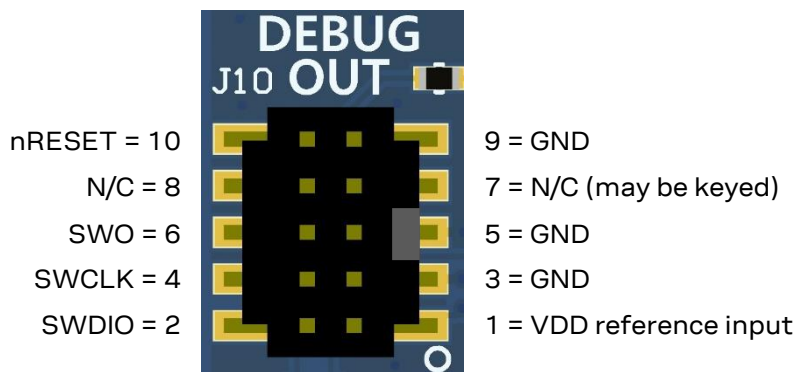
Figure 13: Cortex-M debug connector pin out on EVK-NORA-B1 for SWD
