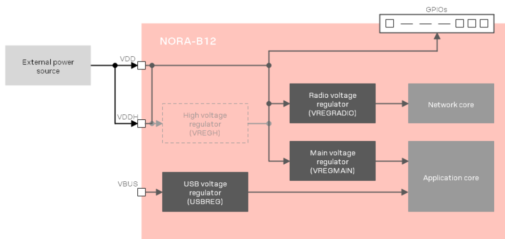
Figure 5: NORA-B12 power connection
