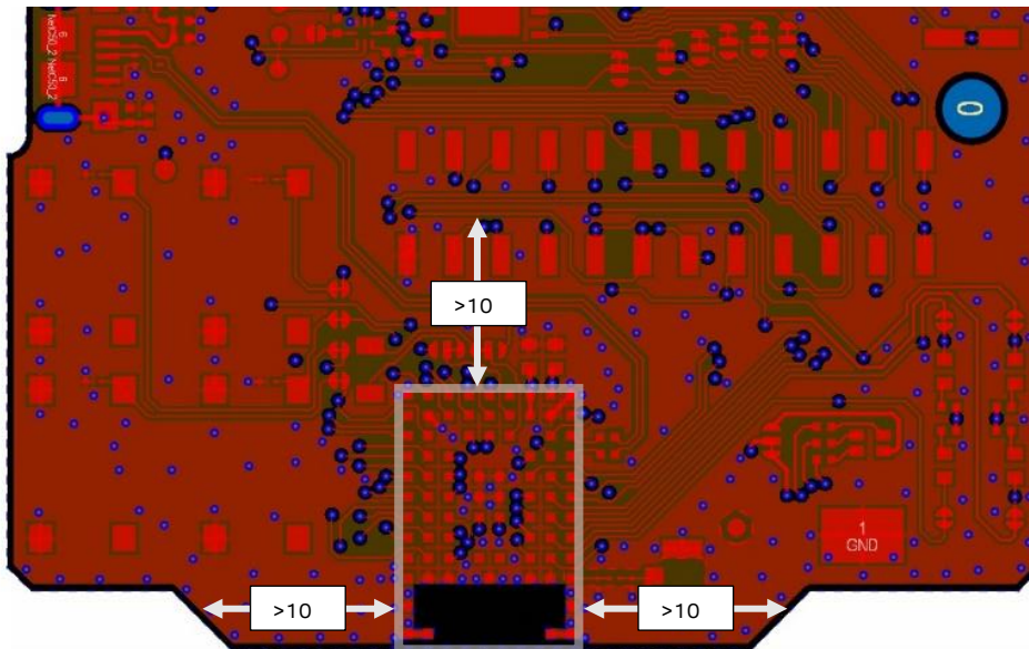
Figure 11: Extend GND plane outside the NORA-B106 and NORA-B126 modules
