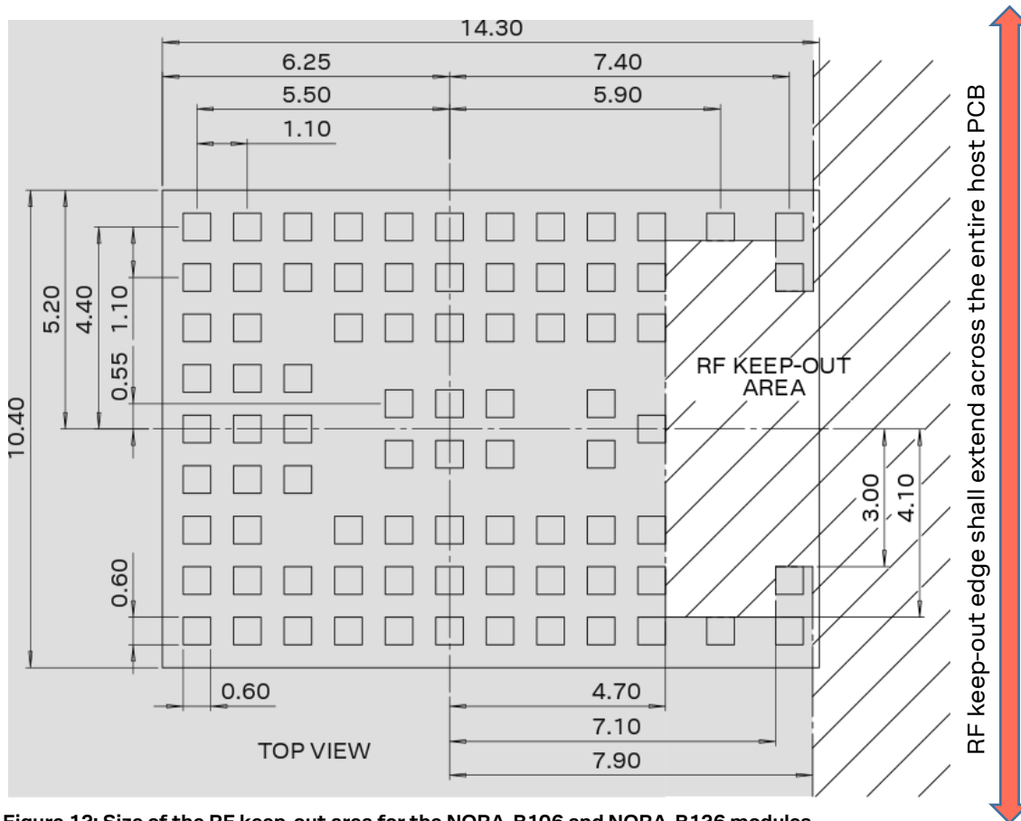
Figure 12: Size of the RF keep-out area for the NORA-B106 and NORA-B126 modules
