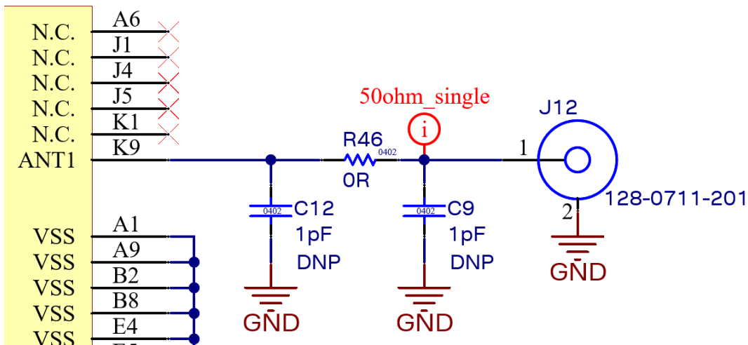
Figure 29: NORA-B101 and NORA-B121 ANT pin U.FL schematic
