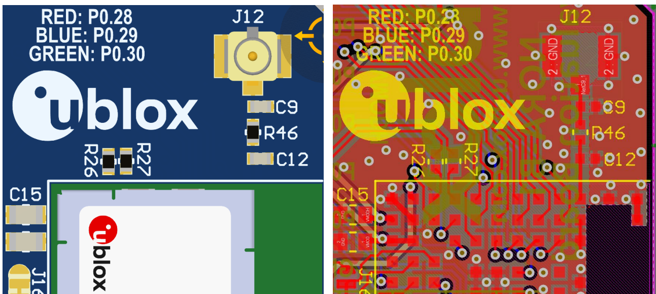
Figure 30: NORA-B101 and NORA-B121 U.FL PCB layout
