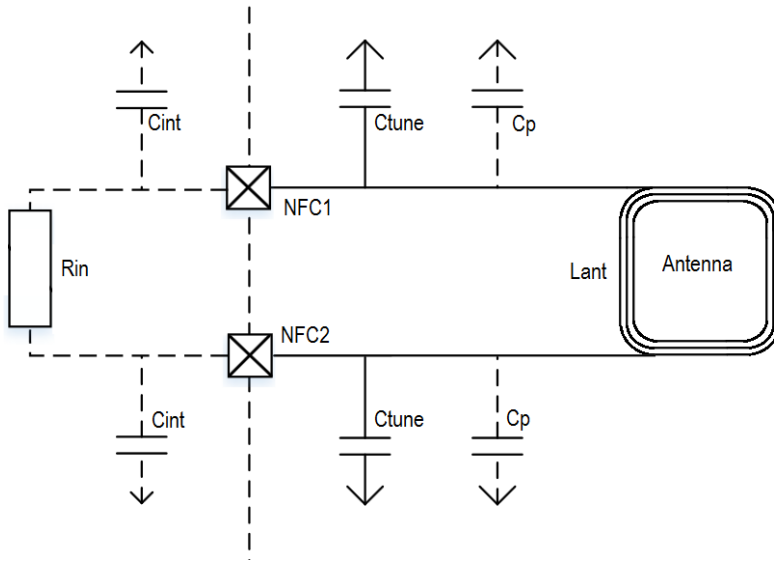
Figure 15: NFC antenna design
