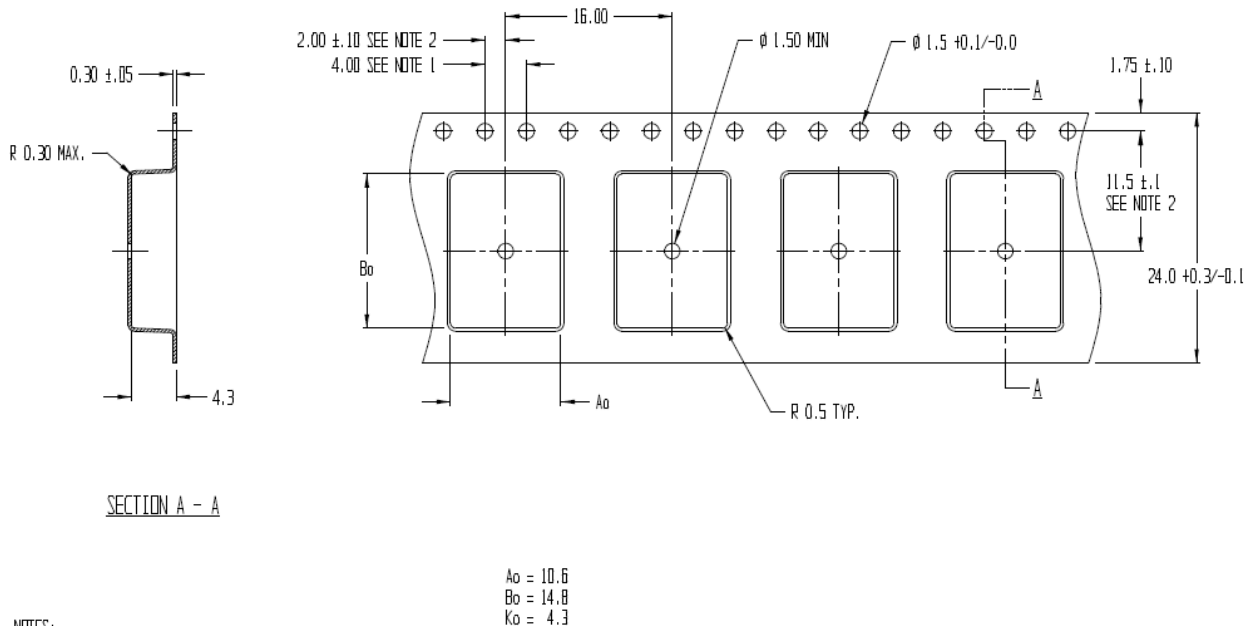
Figure 15: NINA-W151 tape dimension
