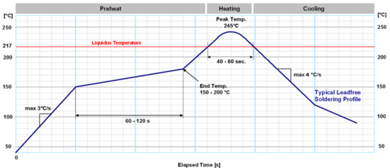
Figure 30: Soldering profile for professional grade NEO-D9S
