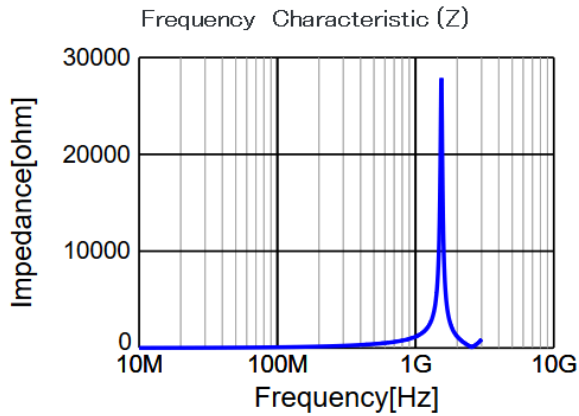
Figure 15: NEO-D9S antenna bias inductor impedance
