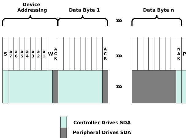
Figure 8: I2C write access
