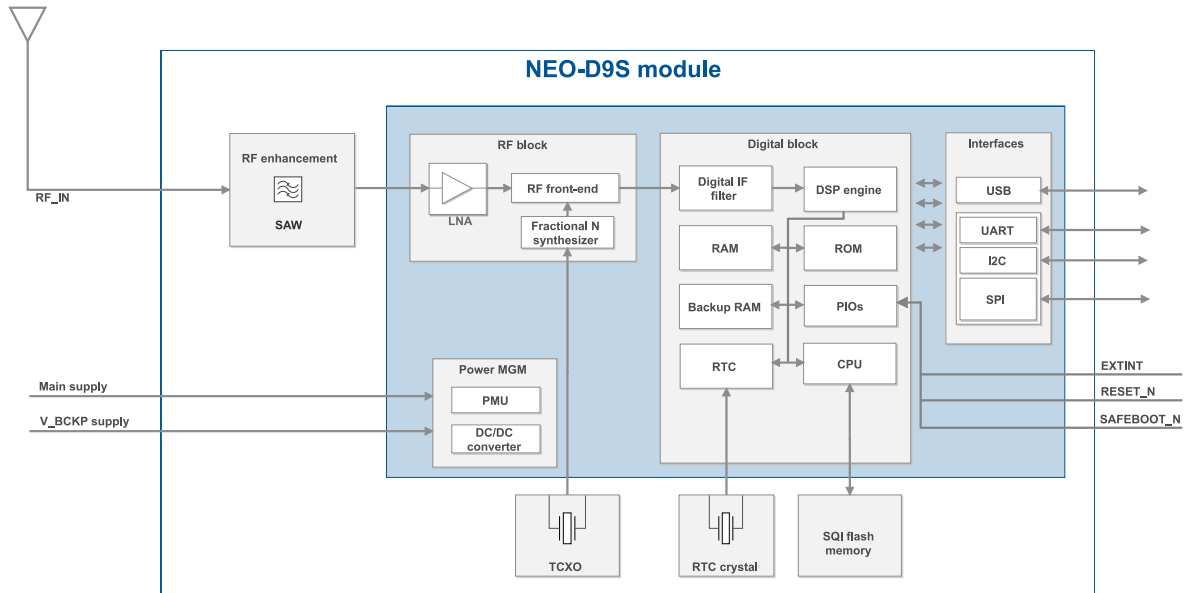
Figure 1: NEO-D9S block diagram
