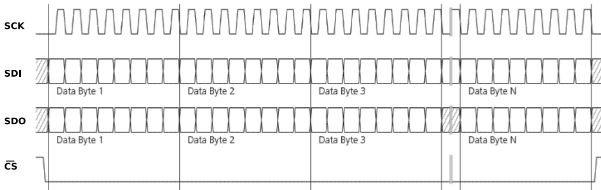
Figure 9: SPI back-to-back read/write access
