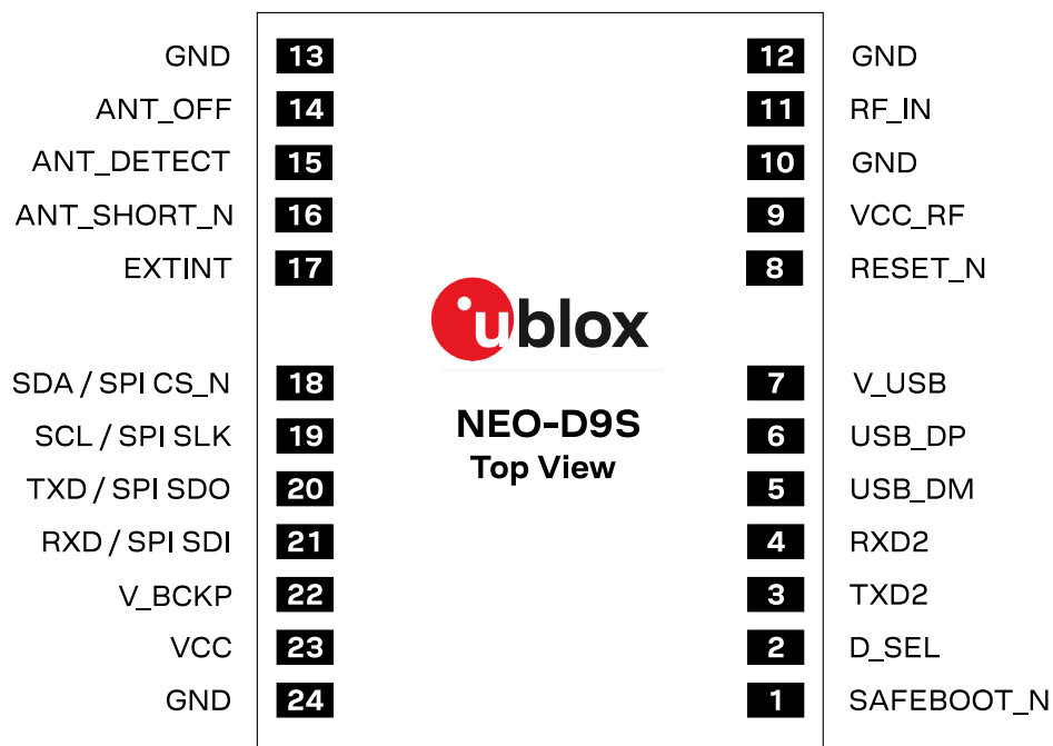
Figure 12: NEO-D9S pin assignment
