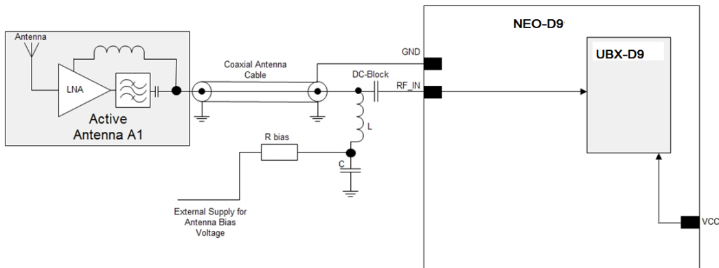
Figure 18: NEO-D9S external voltage antenna bias
