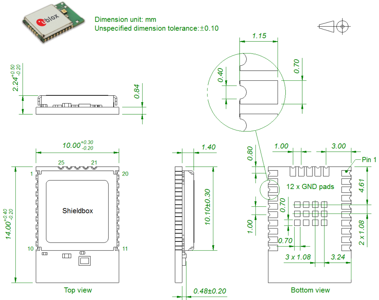
Figure 4: LILY-W131 dimensions
